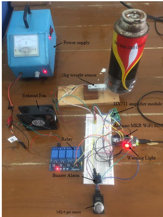
Fig.11. Prototype of LPG Gas Level Detection & Gas Leakage Accident Prevention with Alert System
