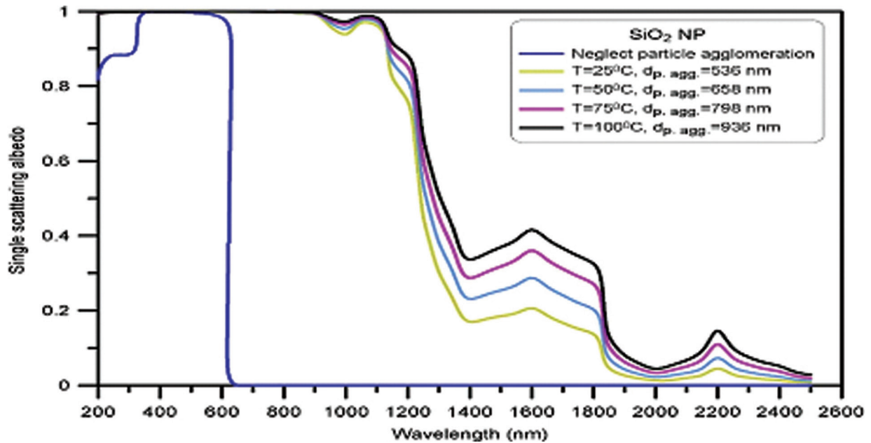
Figure 10. Single scattering albedo of water-SiO 2 nanofluids with different particle agglomerates size.
