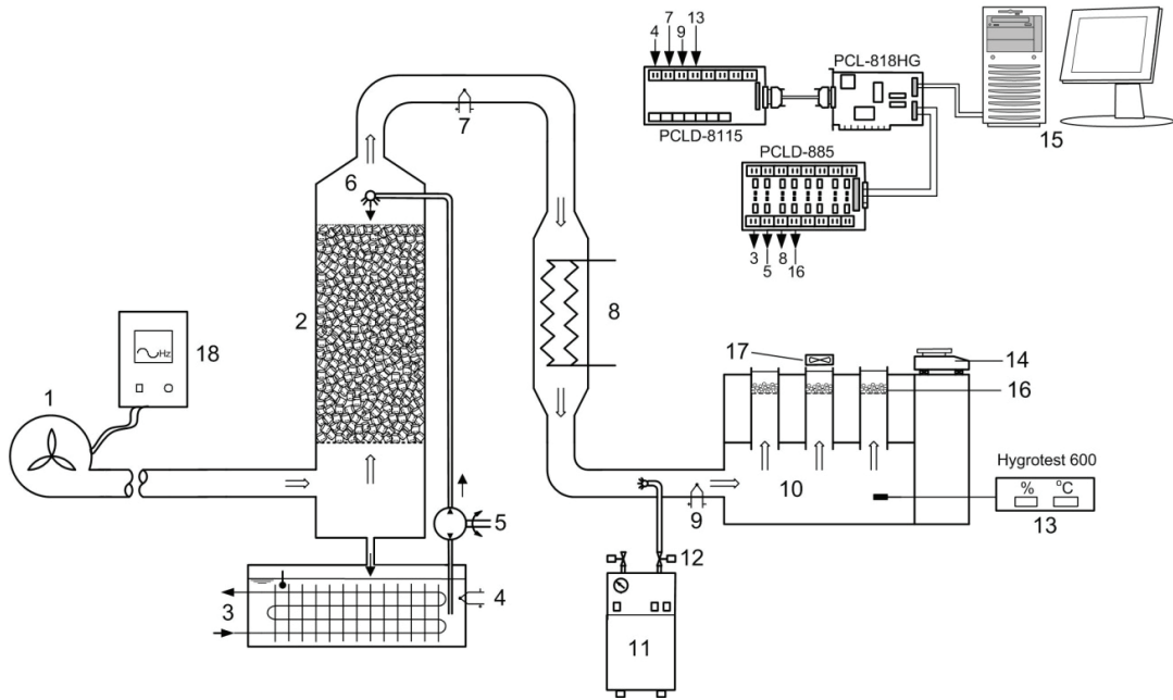
Figure 1- Schematic diagram of the drying unit: 1, centrifugal fan; 2, cooling and condensing tower; 3, cold water tank and evaporator; 4,7,9, thermocouples (type T); 5, circulation pump; 6, cold water shower; 8, electric heaters; 10, mixing chamber and air channels; 11, steam tank; 12, solenoid valve; 13, temperature & humidity sensor; 14, balance; 15, computer with data acquisition and control cards; 16, artichoke leaves; 17, anemometer; 18, frequency converter
