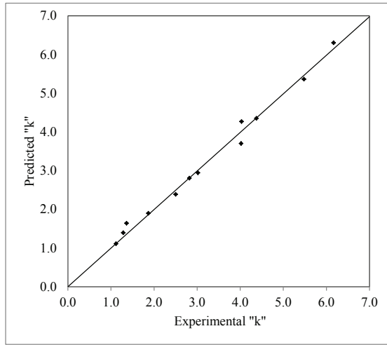
Figure 4- Comparison of the experimental and predicted drying constant ( k ) of the Midilli et al model
