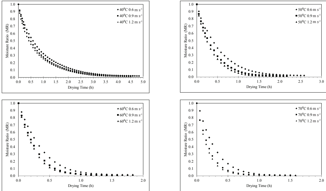
Figure 2- Variations of moisture ratio as a function of time for different air-drying temperatures and velocities
