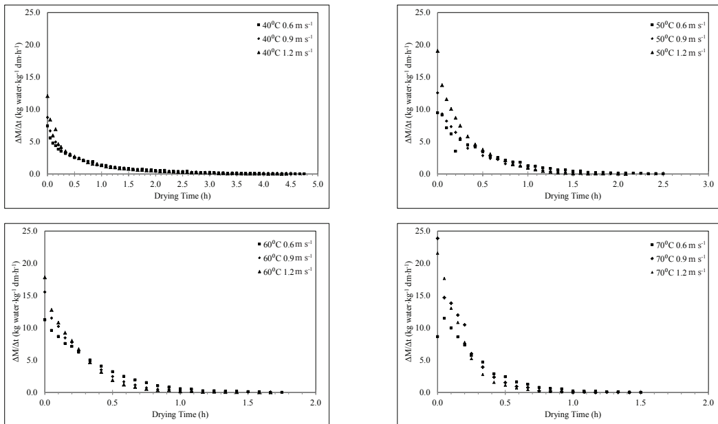
Figure 3 - Variations of drying rate as a function of time for different air-drying temperatures and velocities
