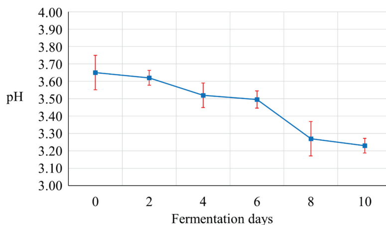
Figure 1- Change in pH during hardaliye fermentation
