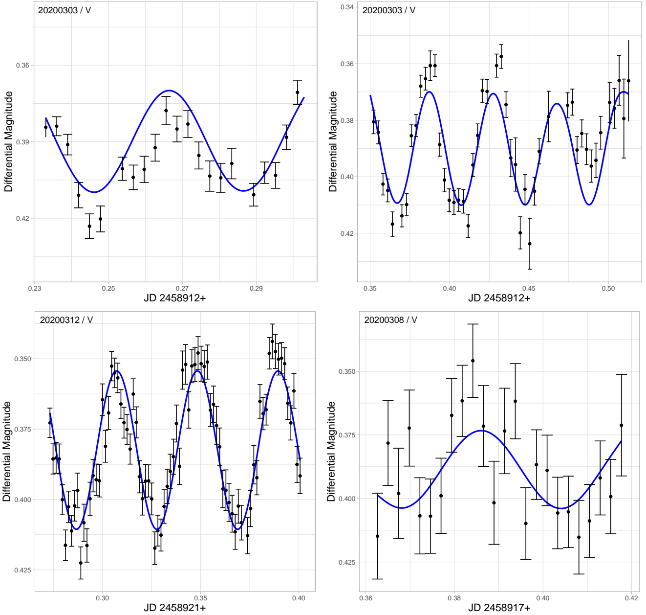
Figure 6. V-band light curves of the candidate variable. Model curves (blue lines) obtained from the period analysis are also plotted. Details of the maxima times and periods are given in Table 3 and 4.
