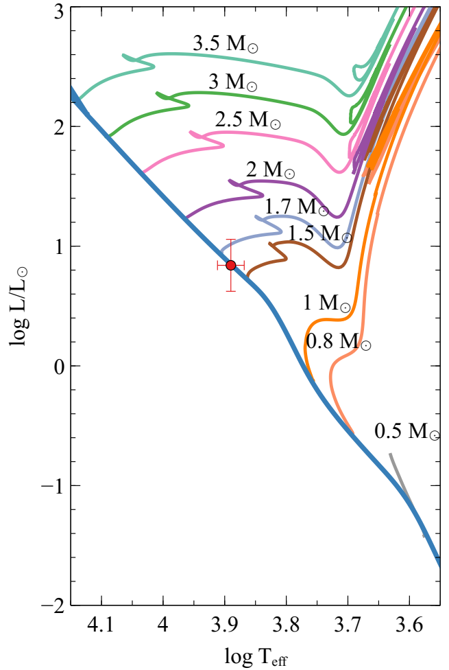
Figure 9. Evolutionary tracks for low-mass stars computed with MESA codes (Paxton et al. 2011). The location of the variable is marked with a red point which is between the tracks of 1.5–1.7 M_{\odot} stars. Error on the luminosity comes from the period-luminosity relation and the bolometric correction whereas the error on the effective temperature mainly comes from the color index calibration given in Cox (2000).
