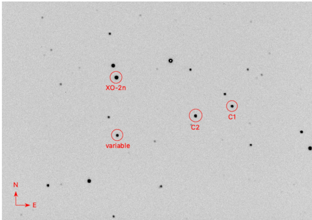
Figure 2. Field of the variable taken from IST40 telescope on the night 23 February 2020. Variable and comparison stars are marked as well as the exoplanet host star XO-2.
