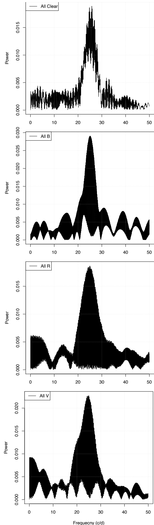
Figure 3. Power spectra for each filter. Plotted frequencies were obtained by combining all available data for the given filter.
