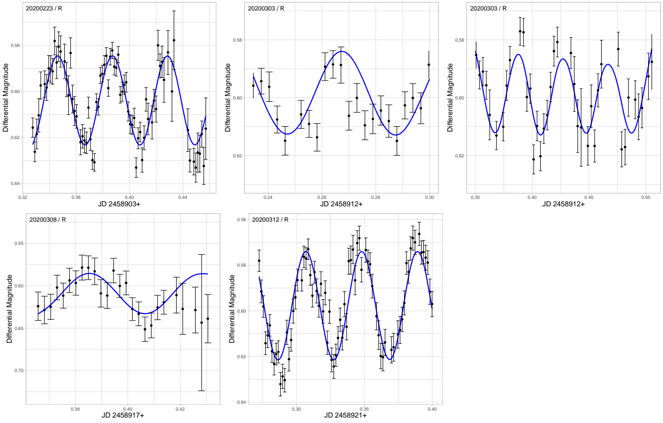
Figure 7. R-band light curves of the candidate variable. Model curves (blue lines) obtained from the period analysis are also plotted. Details of the maxima times and periods are given in Table 3 and 4.
