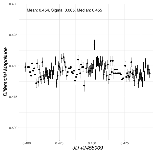
Figure 1. Light curve of C1-C2 difference obtained on 29 February 2020. Frame-to-frame variations of 5 mmag ensure that both comparison stars are not variable.
