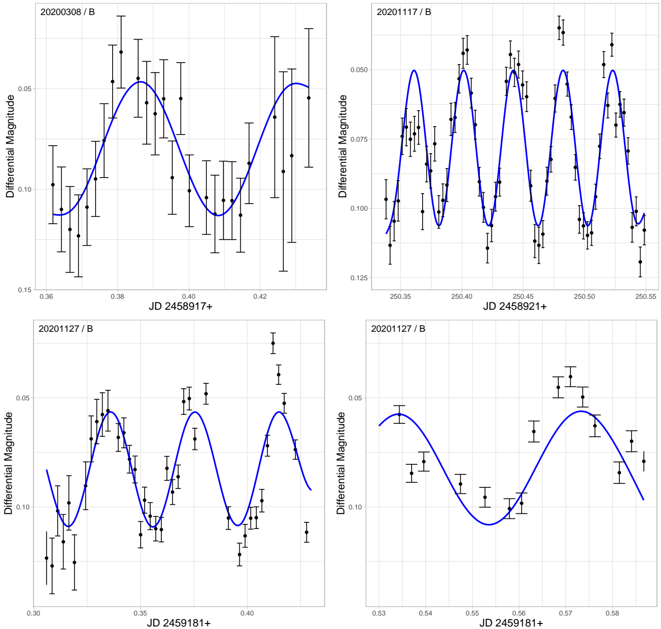
Figure 5. B-band light curves of the candidate variable. Model curves (blue lines) obtained from the period analysis are also plotted. Details of the maxima times and periods are given in Table 3 and 4.
