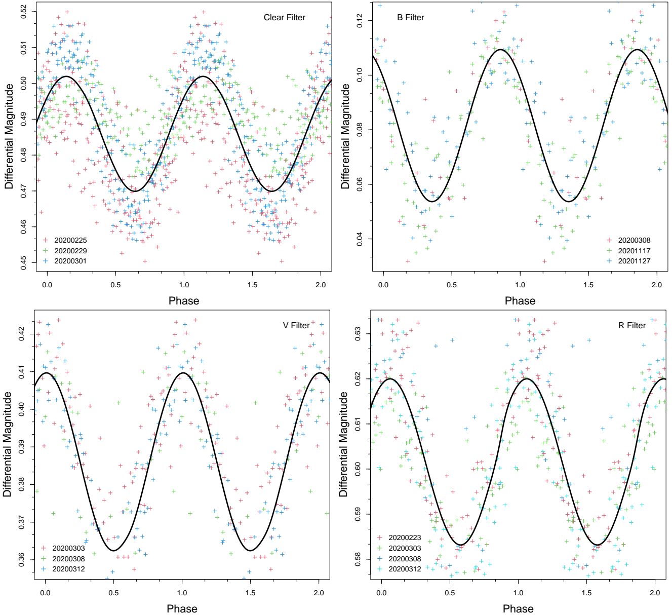
Figure 8. Phase diagram of the time-series data folded on the principal frequency obtained for each filter.
