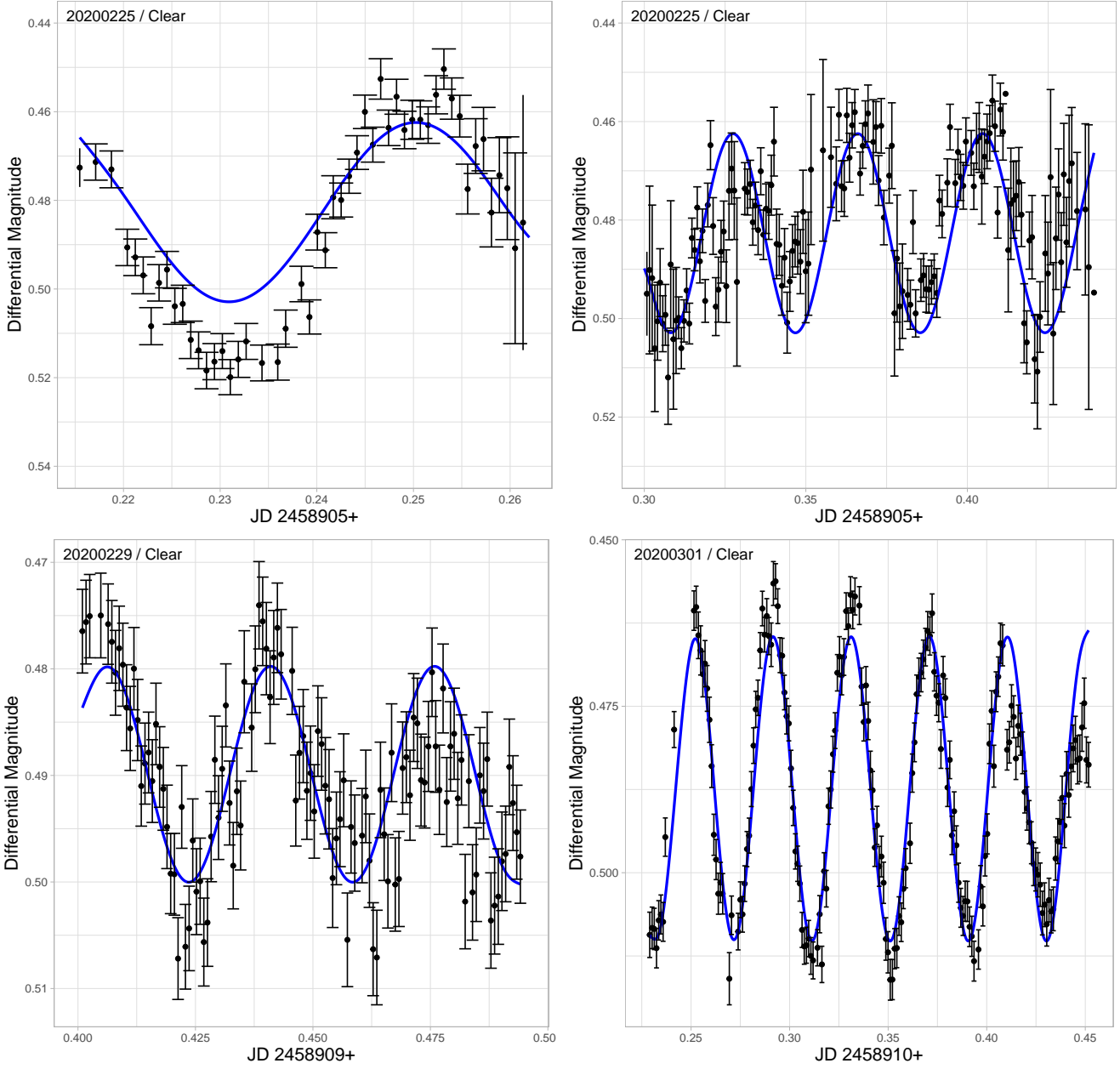
Figure 4. Unfiltered (clear) light curves of the candidate variable. Model curves (blue lines) obtained from the period analysis are also plotted. Details of the maxima times and periods are given in Table 3 and 4.
