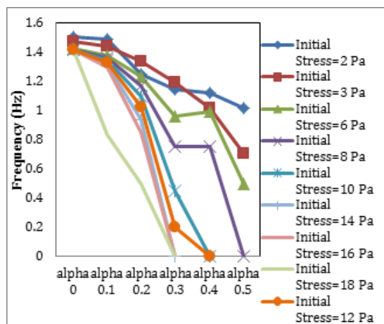
Figure 8. Frequencies of clamped end micro/nano beams
