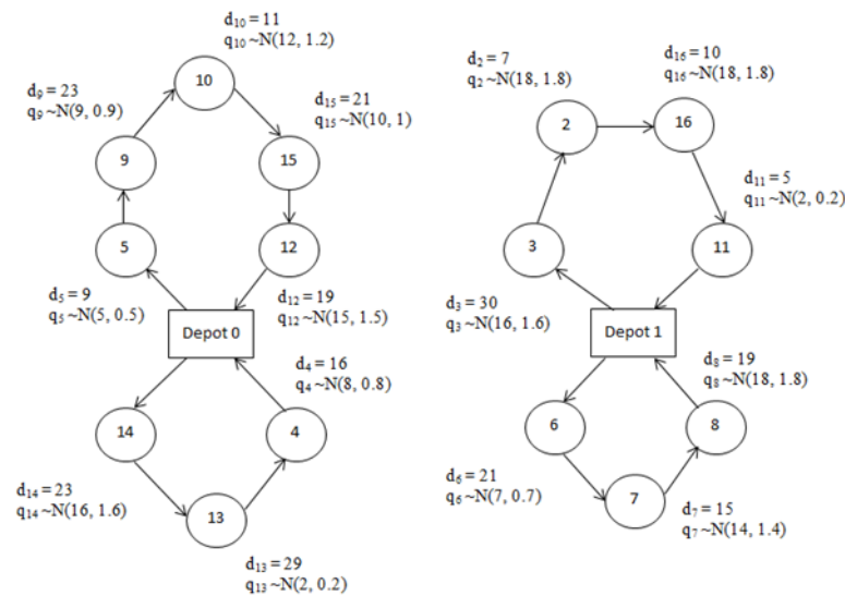
Figure 1. Showing the results obtained from solving the test problem with linearized model on the network
