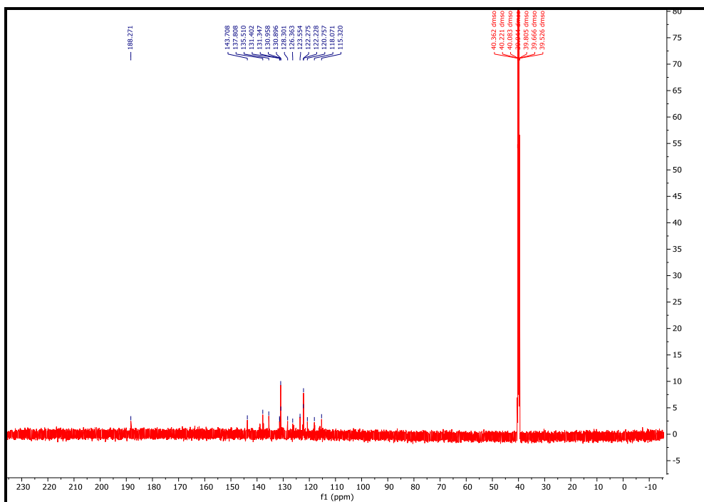
Fig. S5. ^{13}\text{C} NMR spectrum of compound 2
