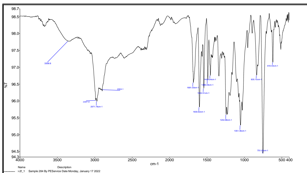
Fig. S1. FTIR spectrum of compound 1
