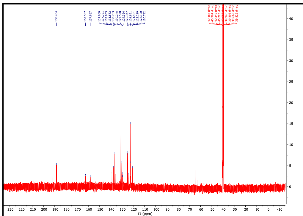
Fig. S16. ^{13}\text{C} NMR spectrum of compound 6
