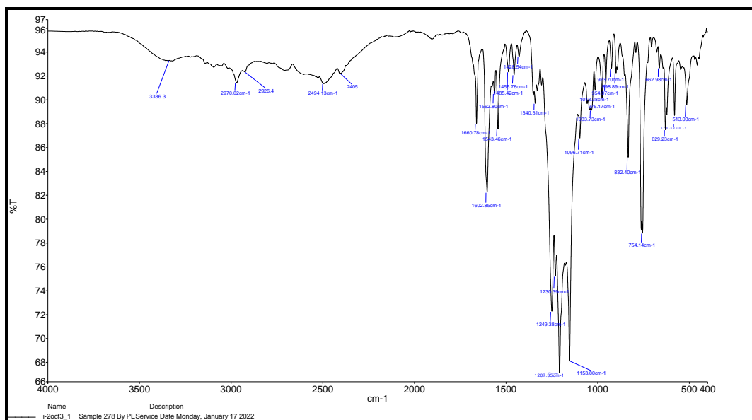
Fig. S25. FTIR spectrum of compound 10
