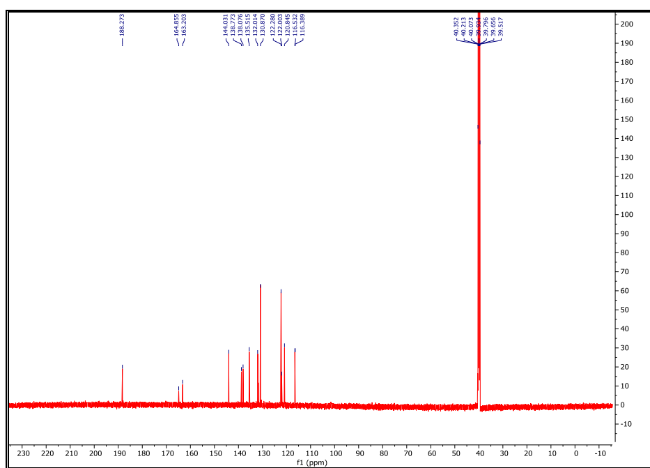
Fig. S8. ^{13}\text{C} NMR spectrum of compound 3
