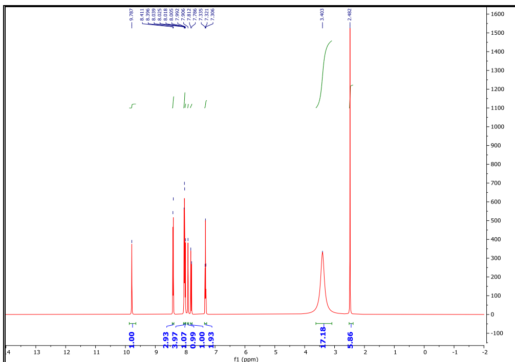
Fig. S7. ^1\text{H} NMR spectrum of compound 3
