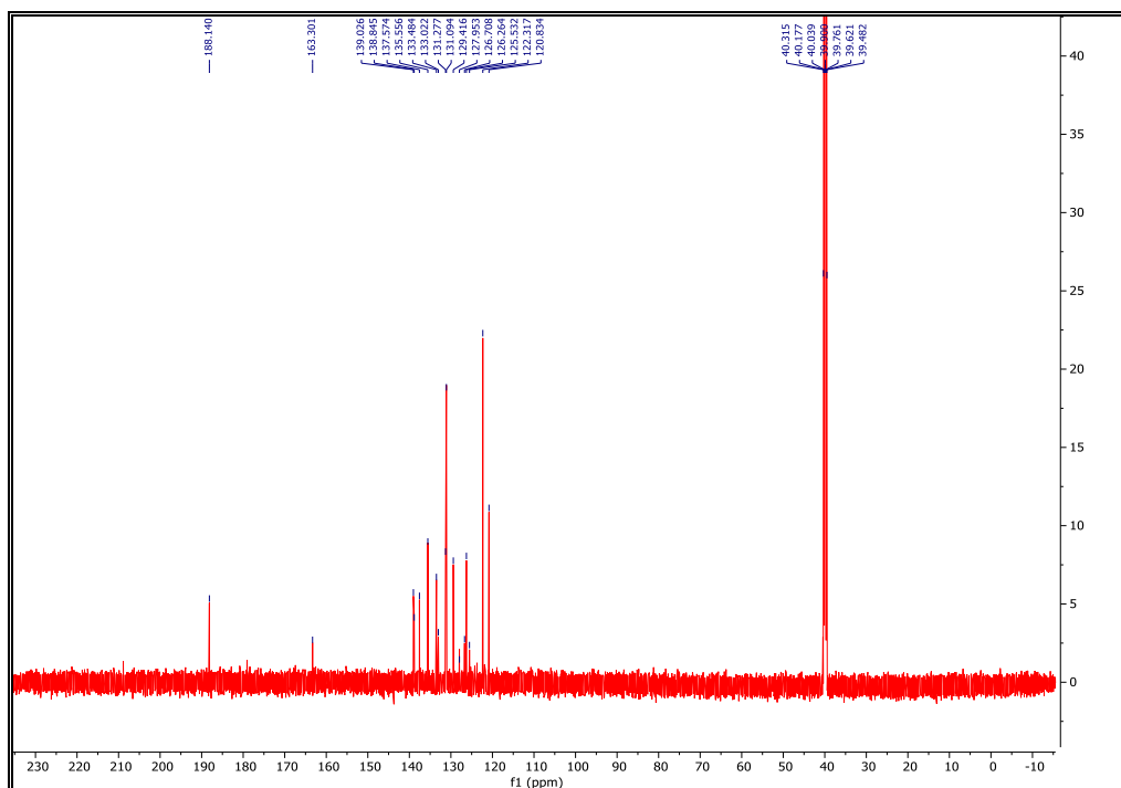
Fig. S11. ^{13}\text{C} NMR spectrum of compound 4
