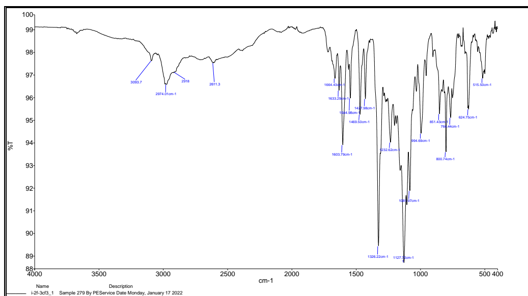
Fig. S14. FTIR spectrum of compound 6
