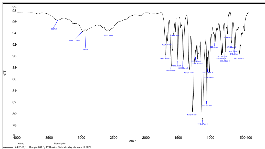
Fig. S19. FTIR spectrum of compound 8
