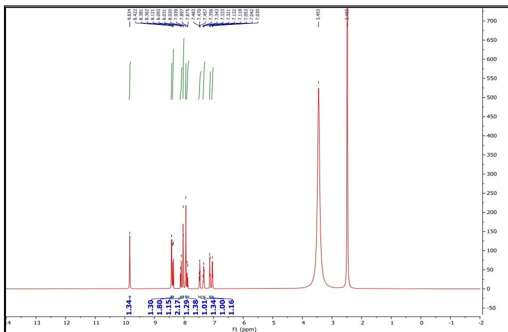
Fig. S2. 1 H NMR spectrum of compound 1
