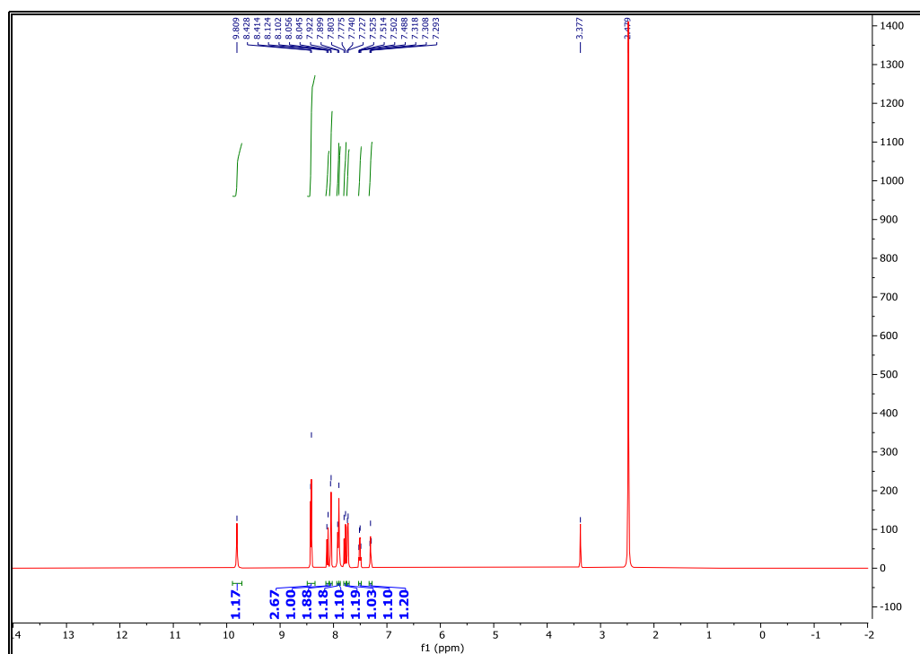
Fig. S4. 1 H NMR spectrum of compound 2
