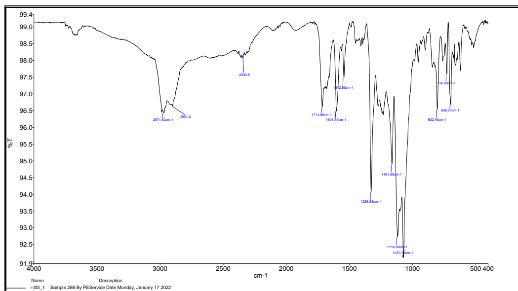
Fig. S12. FTIR spectrum of compound 5
