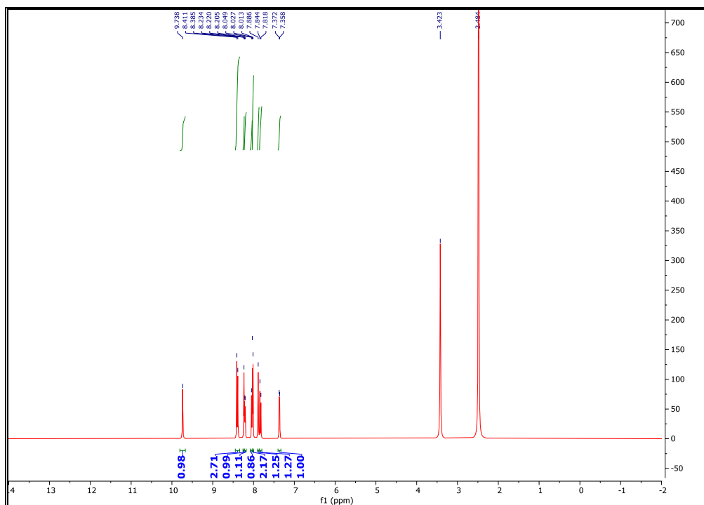
Fig. S23. ^1\text{H} NMR spectrum of compound 9
