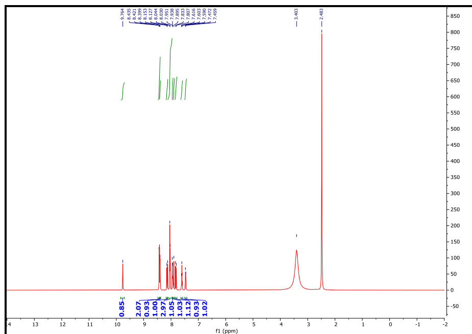
Fig. S29. ^1\text{H} NMR spectrum of compound 11
