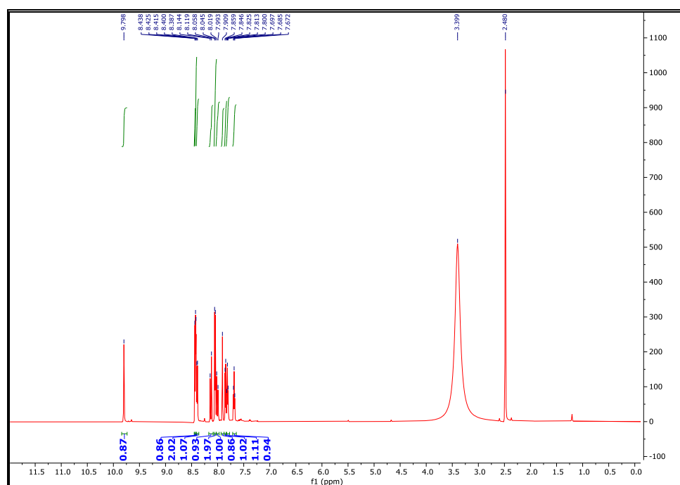
Fig. S10. 1 H NMR spectrum of compound 4
