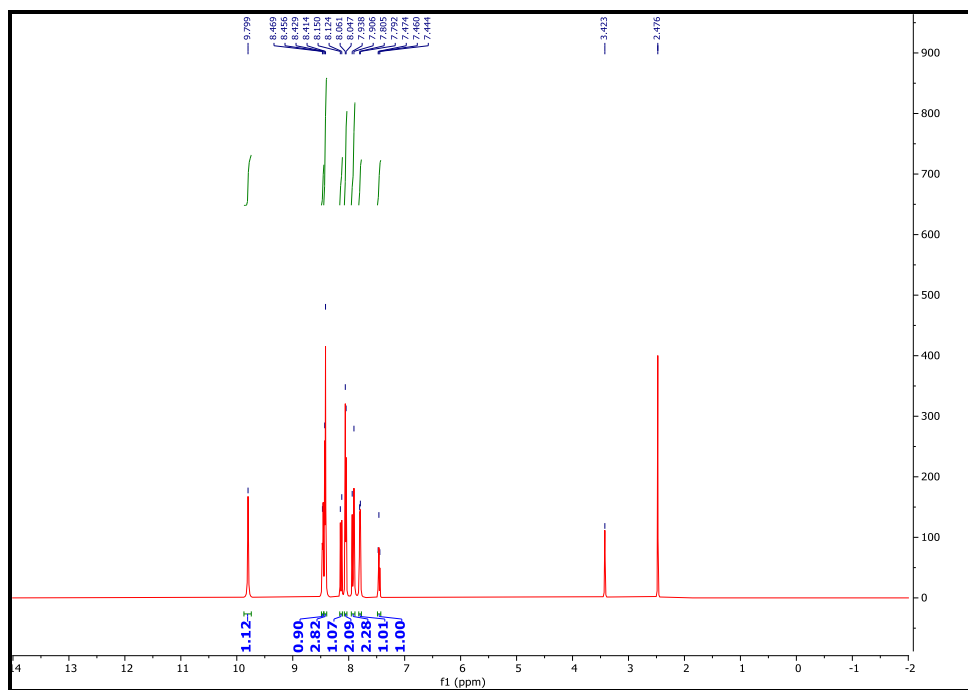
Fig. S15. ^1\text{H} NMR spectrum of compound 6
