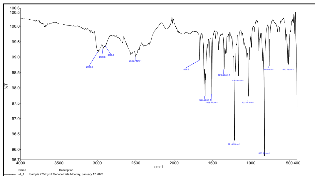
Fig. S6. FTIR spectrum of compound 3
