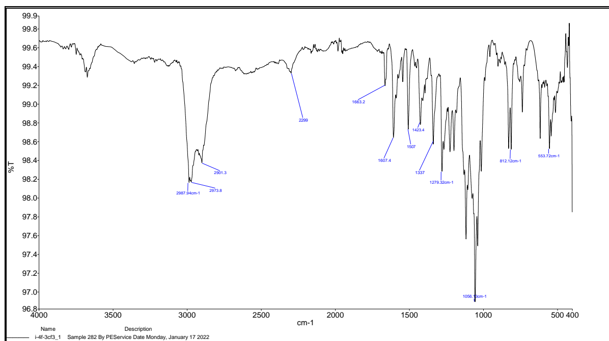
Fig. S22. FTIR spectrum of compound 9
