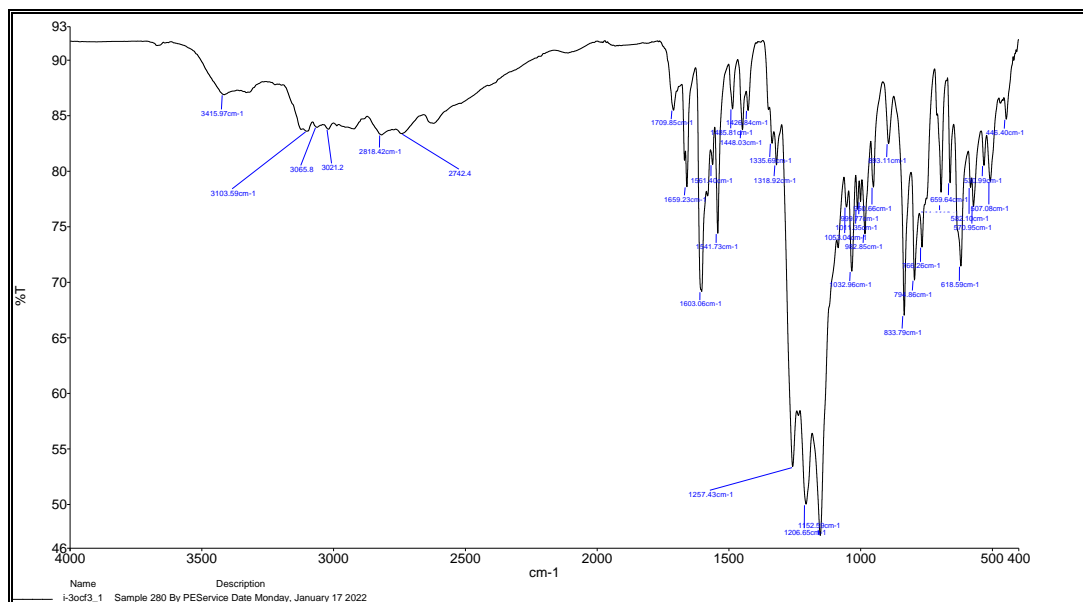
Fig. S28. FTIR spectrum of compound 11
