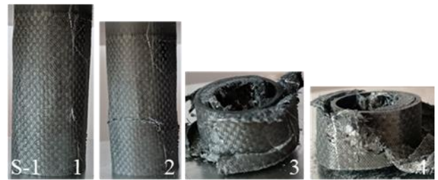
Figure 5. Damage of S-1 specimen during quasi-static compression
