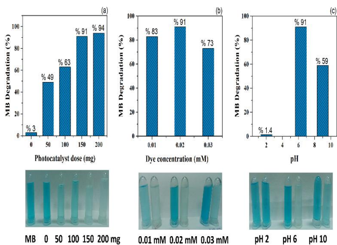
Fig. 3. Effect of (a) catalyst amount, (b) dye concentration and (c) pH on the photocatalytic activity of ZrO 2 nanoparticle.
