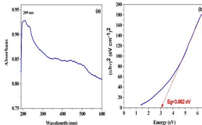
Fig. 2. a) UV-Vis spectrum of ZrO 2 nanoparticles, b) Tauc curve with Kubelka-Munk (K-M) function and estimated band gap of photocatalysis.
