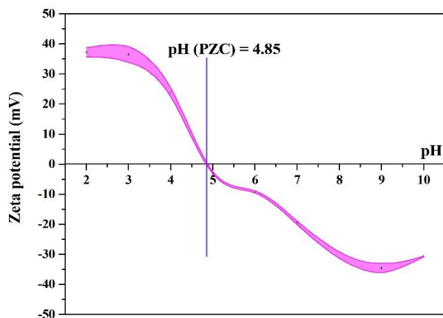
Fig. 1. Zeta potential measurements of ZrO_2 suspension in deionized water
