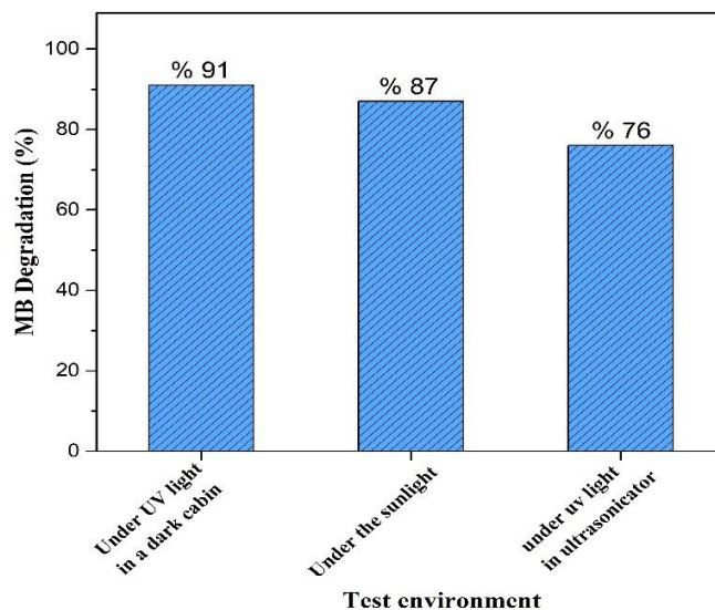
Fig. 5. Effect of test environment on the photocatalytic activity of ZrO 2 nanoparticle
