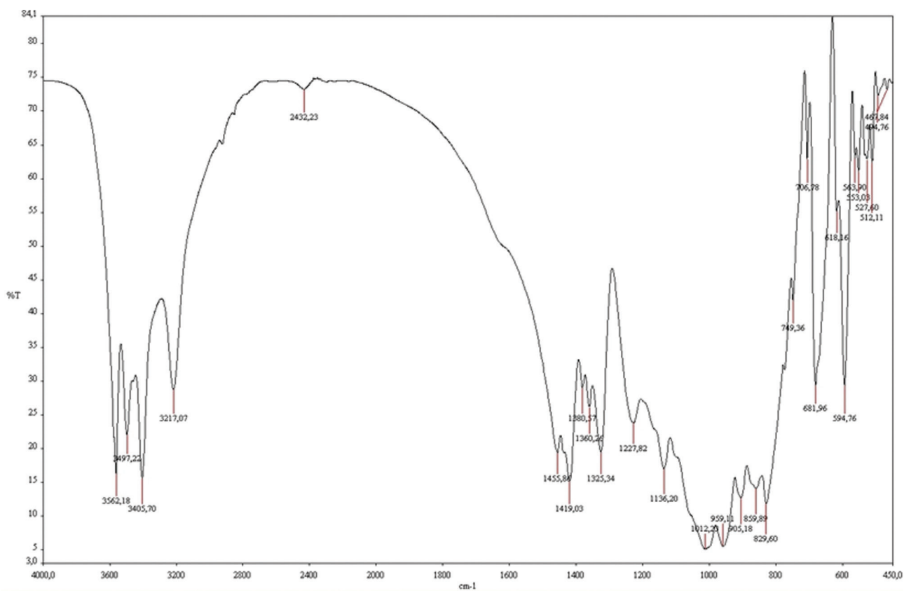
Figure 2. FT-IR spectra of howlite.
