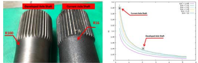
Fig. 7. Comparison of axle shaft transition radius & Kt factors
