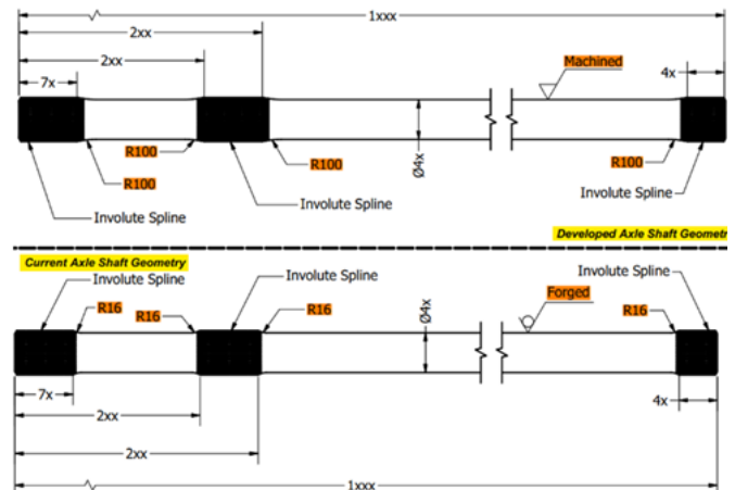
Fig. 4. Geometry of Developed & Current axle shaft
