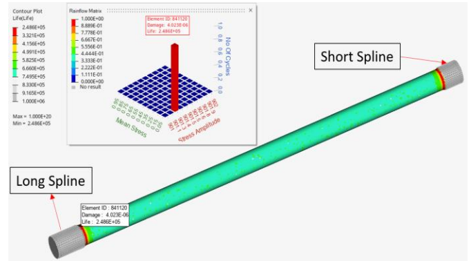
Fig. 18. Current axle FEA cyclic life results
