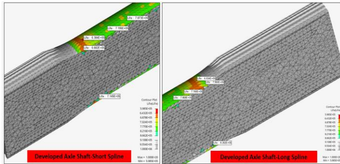
Fig. 21. Developed axle shaft transition zone FEA cyclic life results
