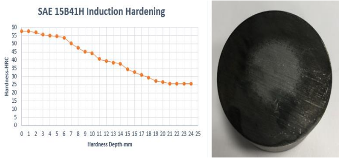
Fig. 5. SAE 15B41H induction hardening
