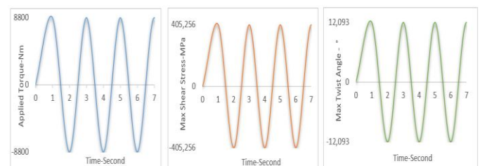
Fig. 9. Torque, shear stress and twist angle diagrams
