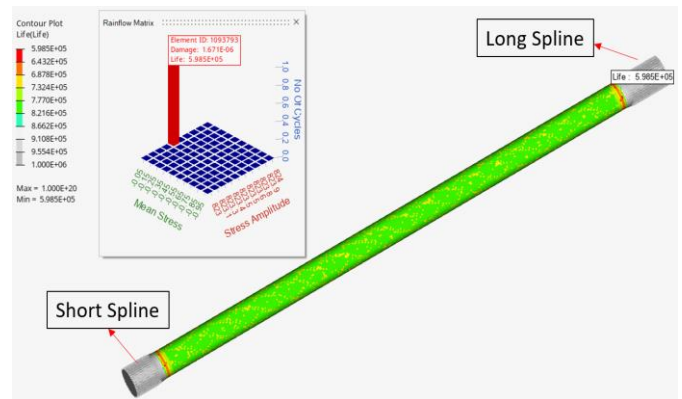
Fig. 19. Developed axle FEA cyclic life results
