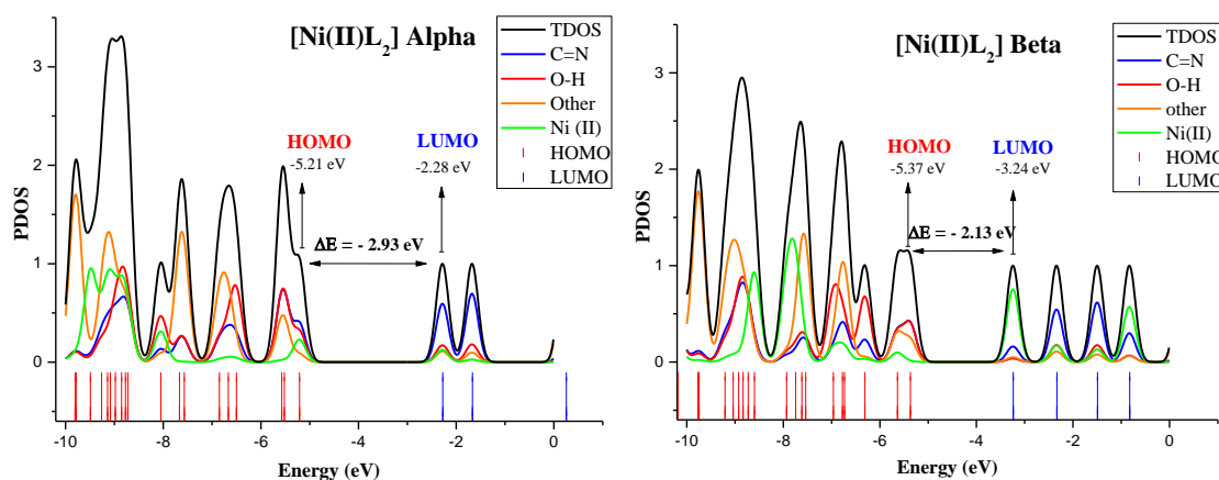
Figure 6. Density of states diagrams (PDOS and TDOS) for the [\text{Ni(II)L}_2] complexes
