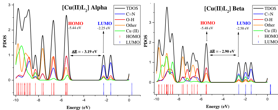
Figure 5. Density of states diagrams (PDOS and TDOS) for the [\text{Cu(II)L}_2] complexes
