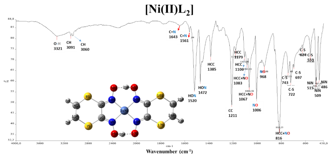
Figure 11. Infrared spectrum of the [Ni(II)L_2]
