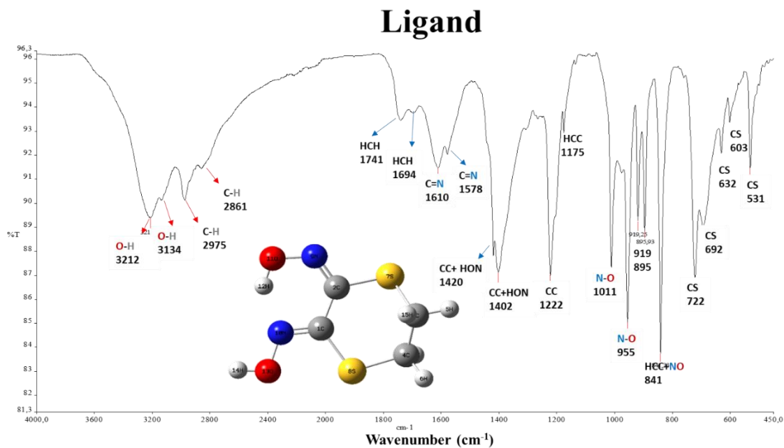
Figure 9. Infrared spectrum of the ligand
