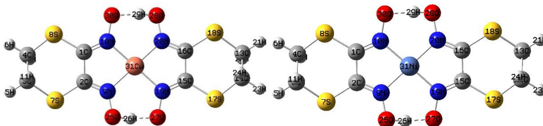
Figure 2. 3D structure of [Cu(II)L 2 ] and [Ni(II)L 2 ] complexes
