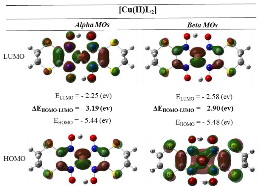
Figure 3. Molecular orbitals and energies of the [Cu(II)L 2 ] complexes
