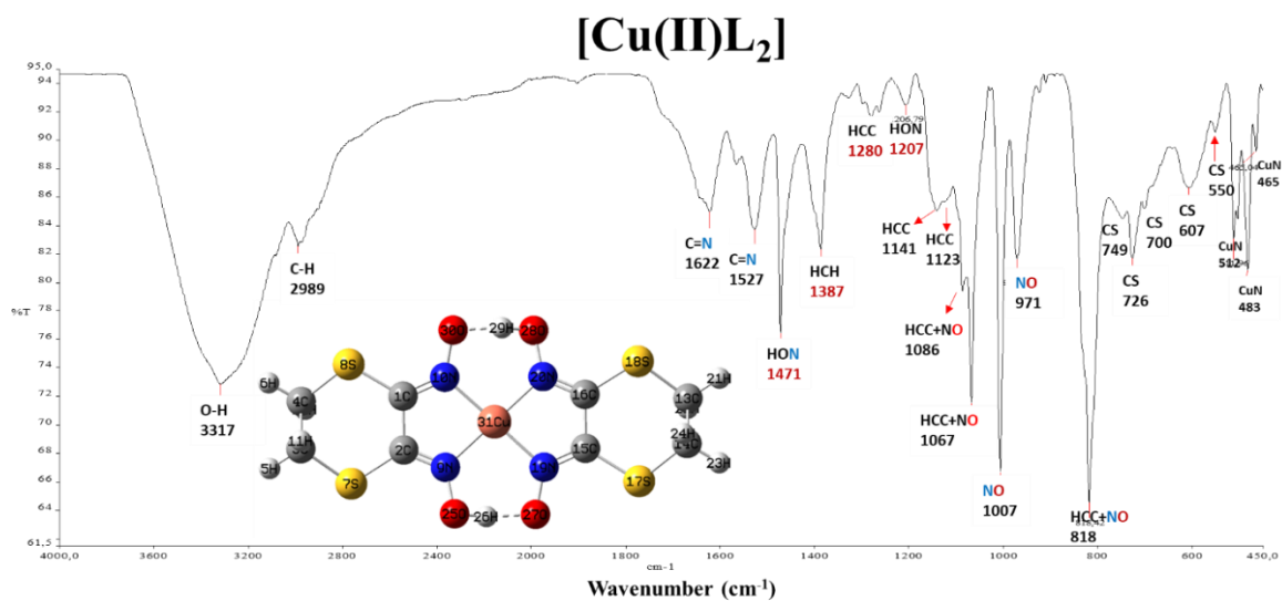
Figure 10. Infrared spectrum of the [Cu(II)L 2 ]
