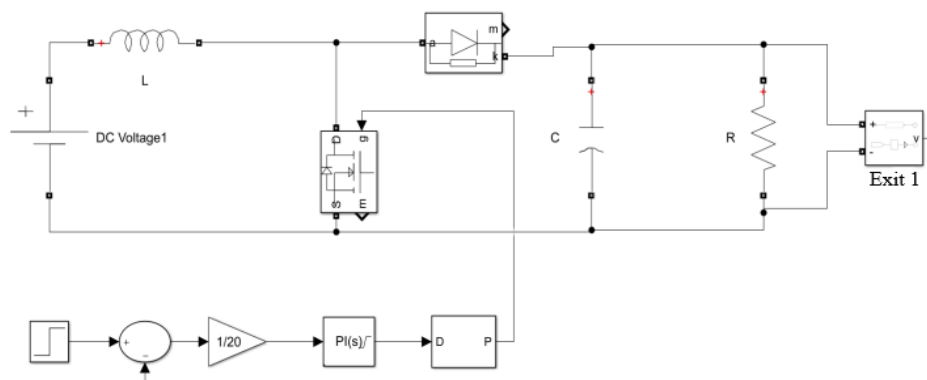
Figure 3. DC-DC boost converter simulation circuit.
