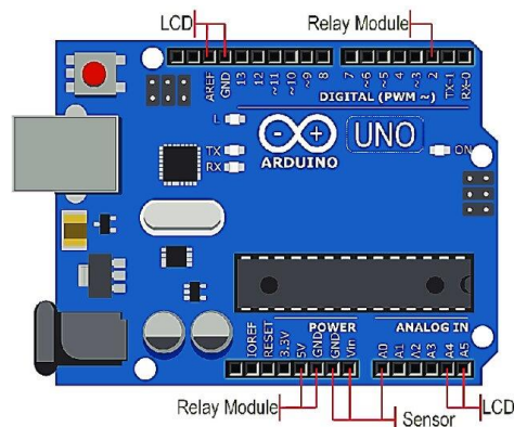
Figure 9. Details of Arduino pin for hardware connection [44].
