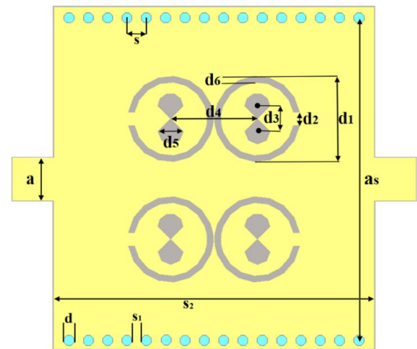
( a=2.0 mm, a_s=15.0 mm, s=900 μm, s_1=400 μm, s_2=14.9 mm, d=500 μm, d_1=4.0 mm, d_2=600 μm, d_3=1180 μm, d_4=4025 μm, d_5=1200 μm, d_6=300 μm)
