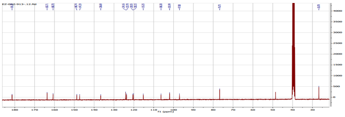
Annexe 8: 1 H and 13 C NMR spectra of compound 8
