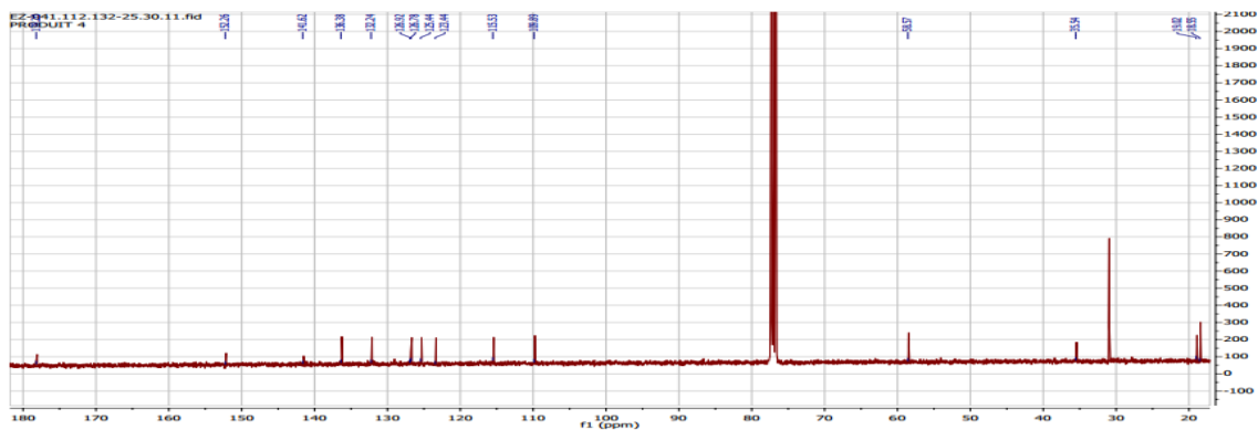
Annexe 3: ^1\text{H} and ^{13}\text{C} NMR spectra of compound 3
