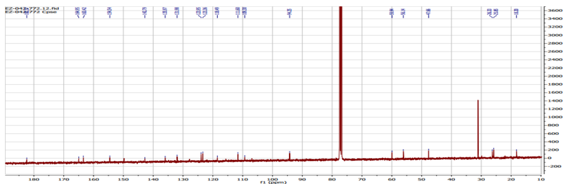
Annexe 6: ^1\text{H} and ^{13}\text{C} NMR spectra of compound 6
