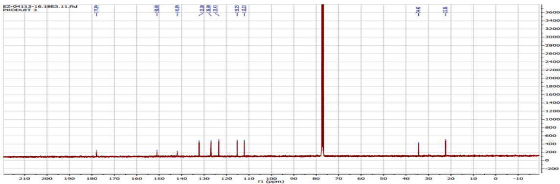
Annexe 4: ^1\text{H} and ^{13}\text{C} NMR spectra of compound 4
