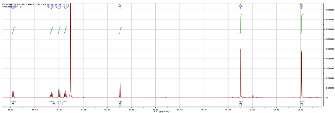
Annexe 3: ^1\text{H} and ^{13}\text{C} NMR spectra of compound 3
