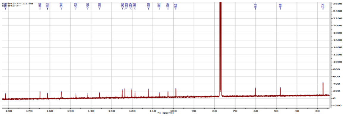
Annexe 7: 1 H and 13 C NMR spectra of compound 7
