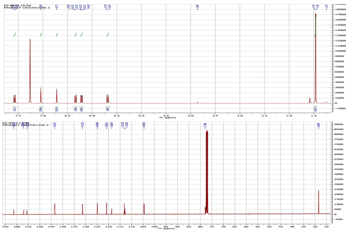
Annexe 1: ^1\text{H} and ^{13}\text{C} NMR spectra of compound 1
