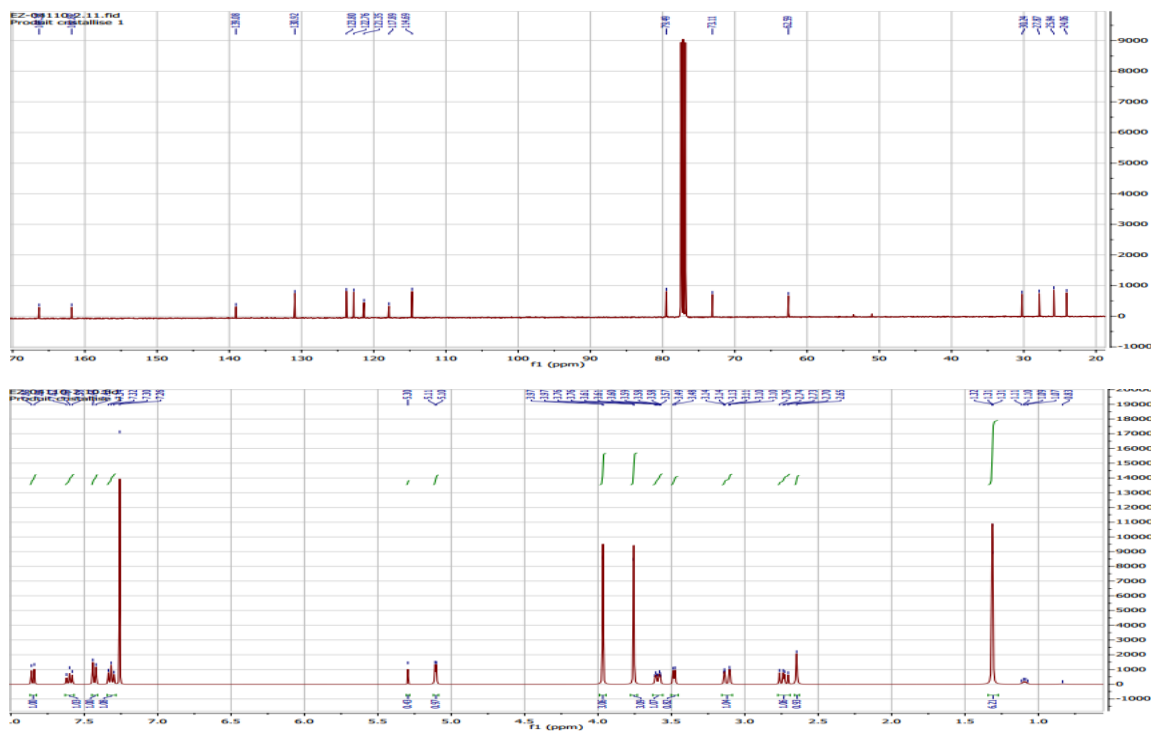
Annexe 2: ^1\text{H} and ^{13}\text{C} NMR spectra of compound 2
