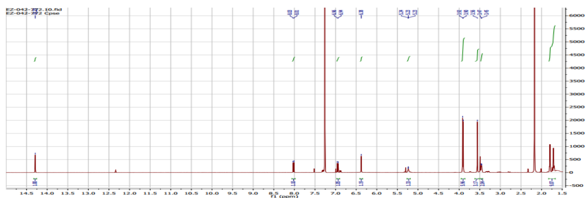
Annexe 5: ^1\text{H} and ^{13}\text{C} NMR spectra of compound 5
