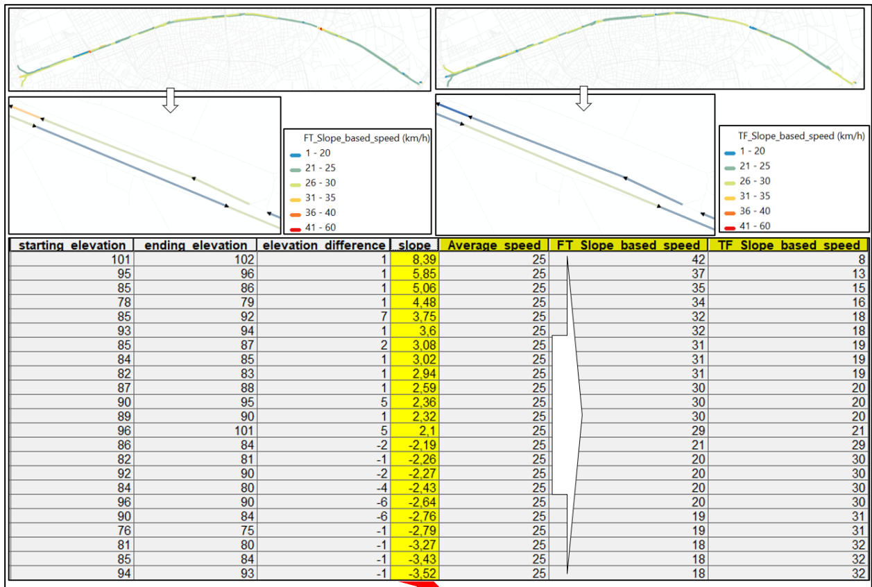
Figure 15. Demonstration of Usability of the Proposed Methodology: An example of cost calibration process for accessibility modelling considering different slope and topological direction (ft speed →from-to speed and tf speed →to-from speed)
