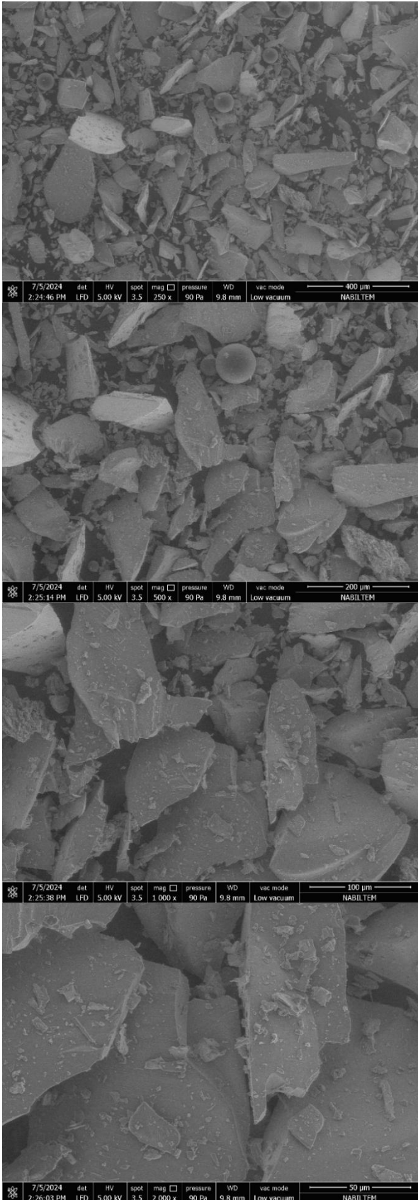
Figure 2. SEM images for WGP (400, 200, 100, and 50 µm)
