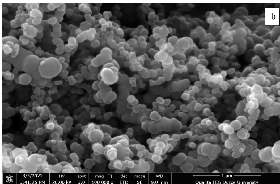
Figure 1. SEM photos of nanoparticles a) \text{TiO}_2 , and b) B.
