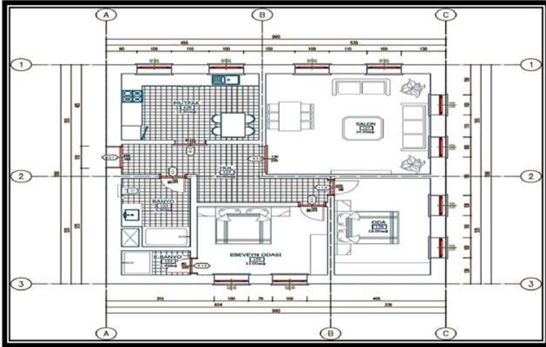
Fig. 4.1. Straw and masonry house, sample house plan prepared for heat and efficiency cost analysis
