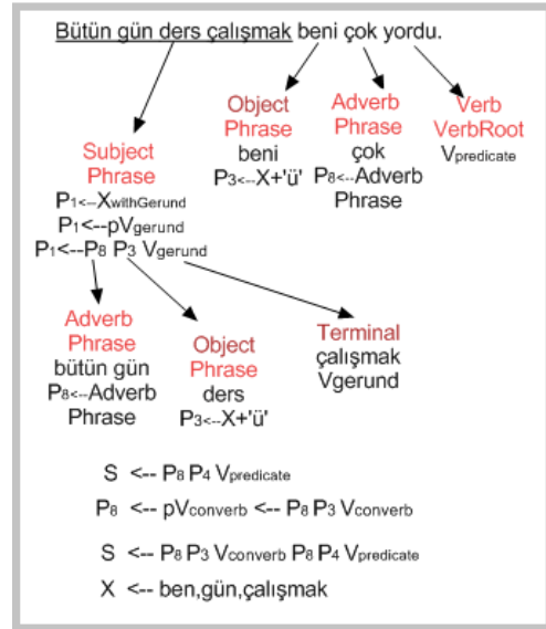
Figure 8. Parsing complex sentence including gerund
