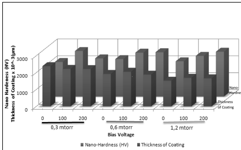
Figure 4.4. Graph of TiAlN coatings' nano-hardness and coating thickness
