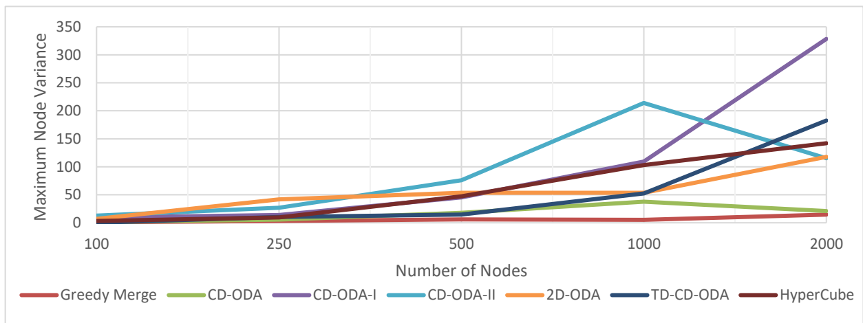
Figure 5. Max. Node Variance for Varying Number of Nodes
