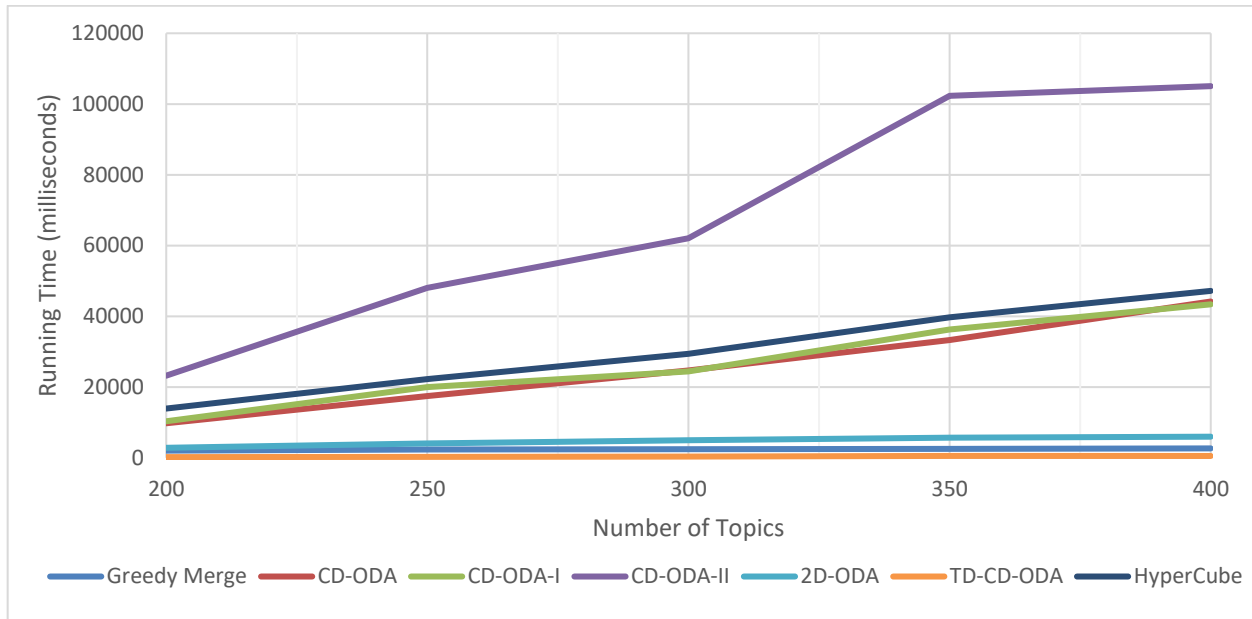
Figure 16: Execution Times for Varying Number of Topics
