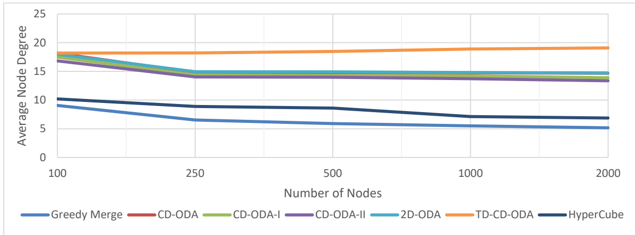
Figure 2. Avg. Node Degree for Varying Number of Node
