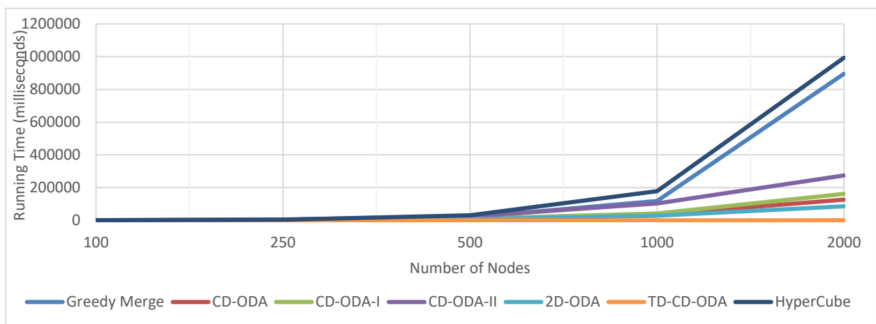
Figure 15: Execution Times for Varying Number of Nodes
