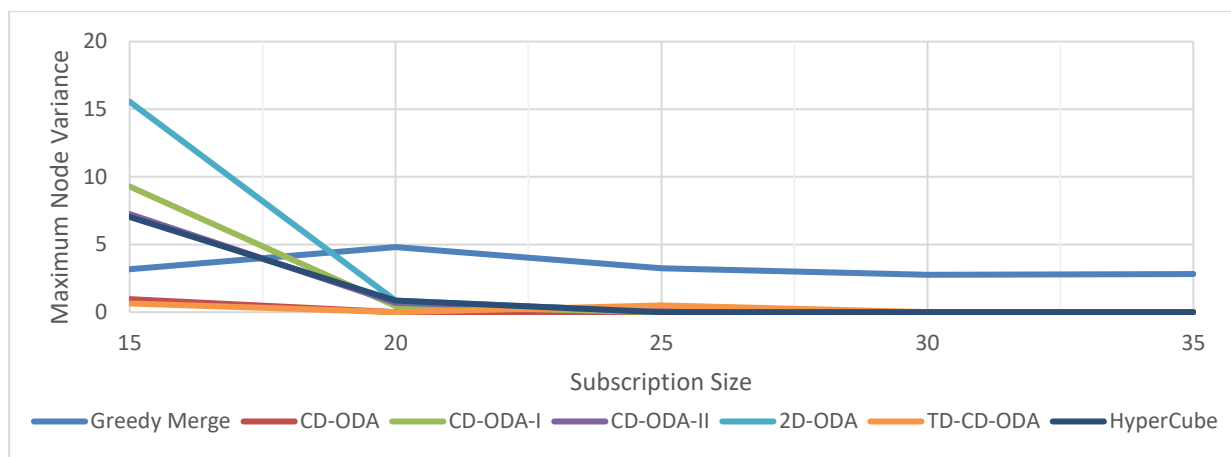
Figure 13. Maximum Node Variance for Varying Subscription Size
