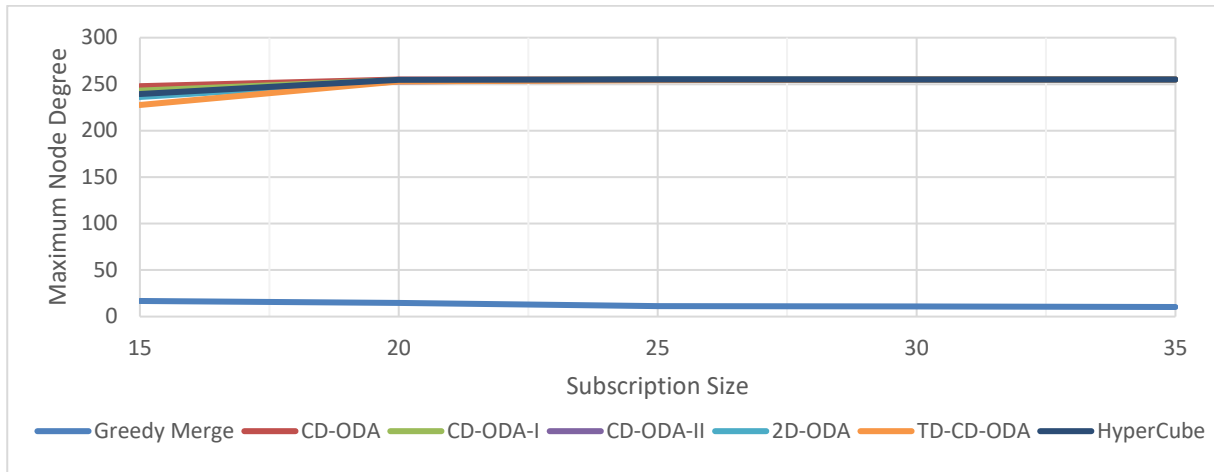
Figure 12. Maximum Node Degree for Varying Subscription Size
