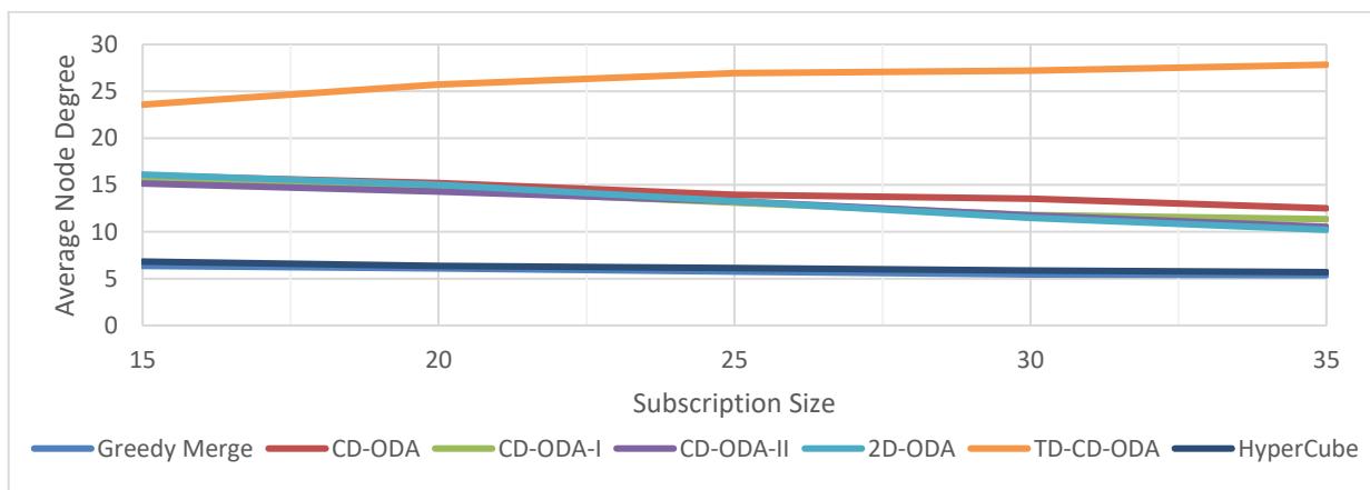
Figure 10. Avg. Node Degree for Varying Subscription Size
