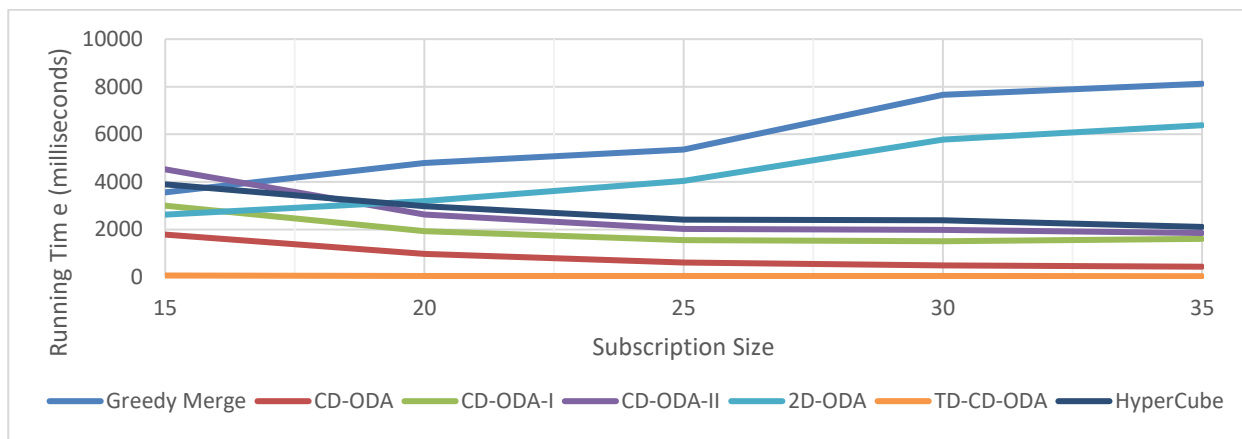
Figure 14. Execution Times for Varying Subscription Sizes
