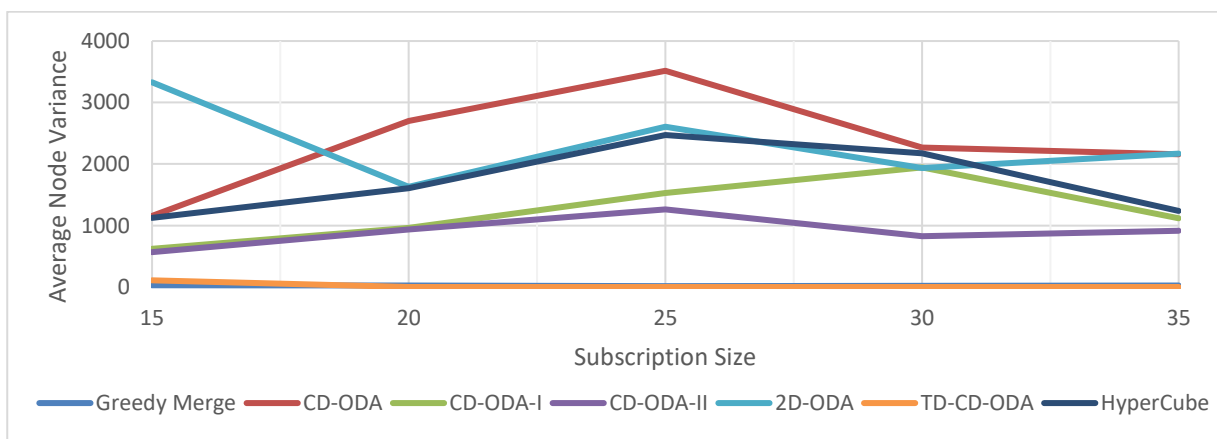
Figure 11. Avg. Node Variance for Varying Subscription Size
