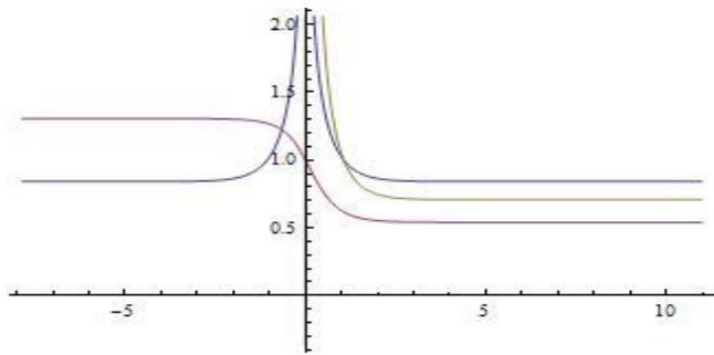
Figure 1: The non-null normal curve in E_2^4
