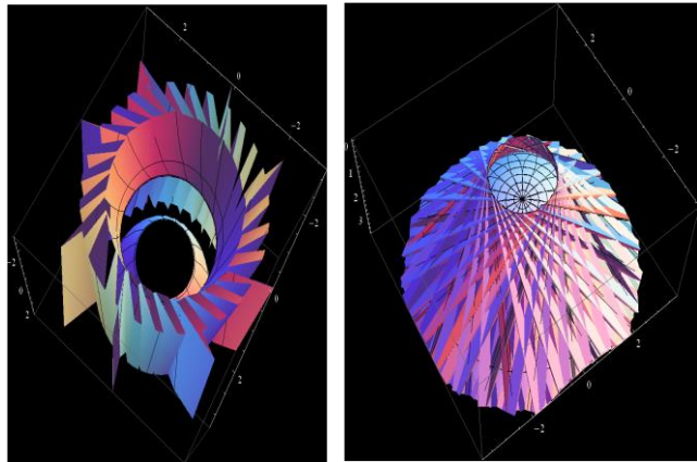
Figure 2: Rotational surfaces generated by the non-null normal curves according to parameters s \in \left(-\frac{5\pi}{2}, \frac{7\pi}{2}\right) and s \in (-\pi, \pi) .
