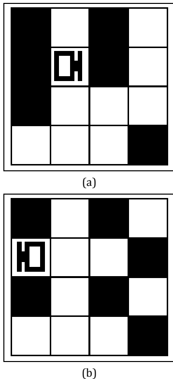
Figure 6. Two boards selected randomly out of 74,760 possible ones.
