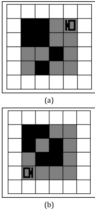
Figure 2(a): Shows the 2 \times 2 formation. (b): Shows a Willson configuration.
