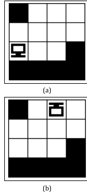
Figure 4. Same distribution of boxes with different starting points creates two very distinct scores. The board in (a): Has an average score of 0.99, and (b): Has an average score of 8.36.
