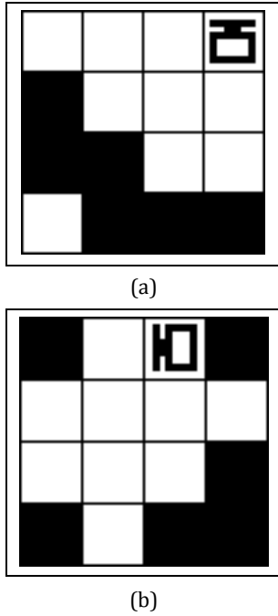
Figure 3. The board in (a): was the hardest for 864 different agents, getting an average score of 0.43. The board in (b): Was the easiest, getting an average score of 9.53.
