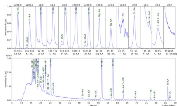
Figure 3. XRF pattern of the volcanic pumice sample.
