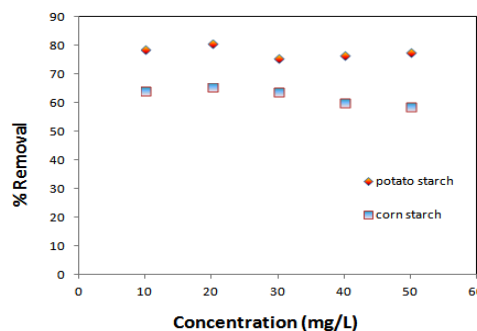
Figure 5. Effect of different beginig concentration of Cu 2+ (pH 5, 0.15 g, 20 min.).
