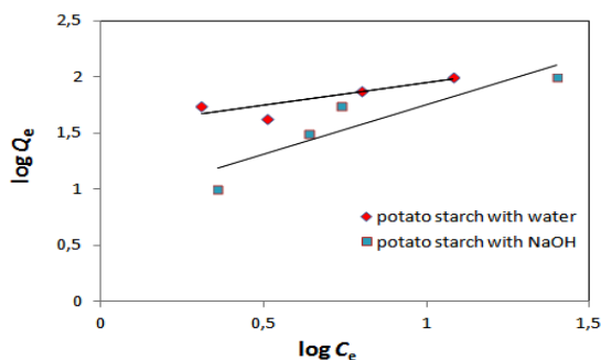
Figure 7. The sorption isotherm of Freundlich which belongs to Cu 2+ ions by using different modification types of potato starch.
