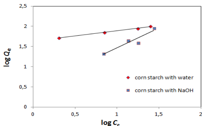
Figure 8. The sorption isotherm of Freundlich which belongs to Cu 2+ ions by using different modification types of corn starch.
