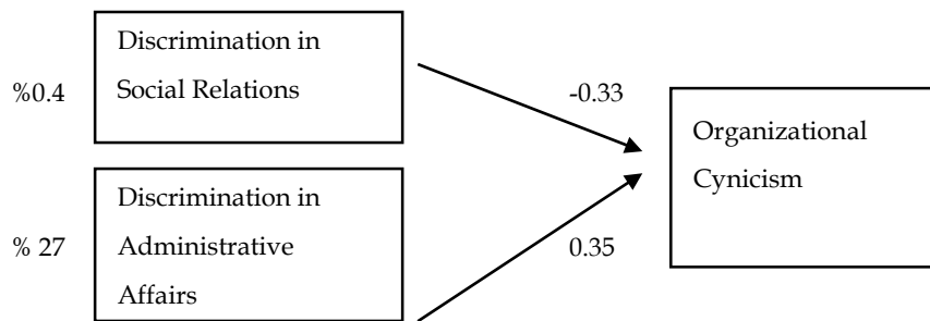
Figure 1. Statistical model
