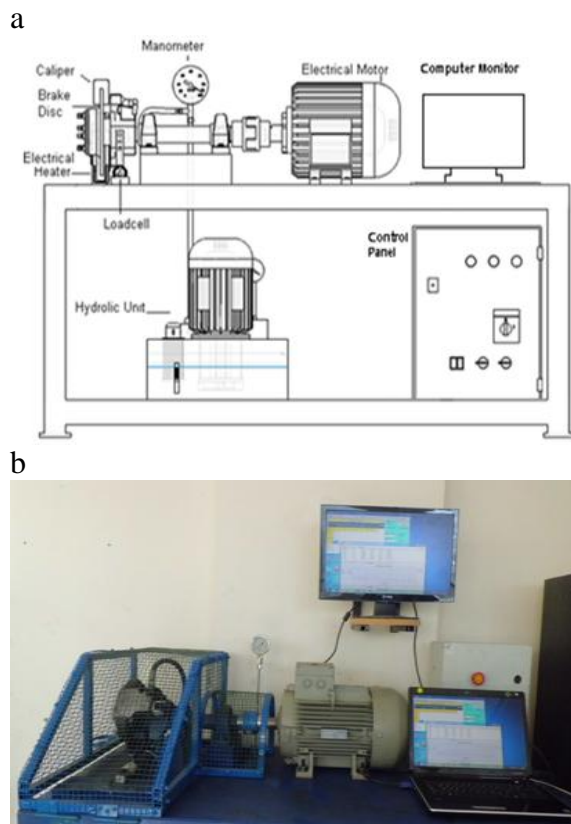
Figure 1. Test set up a) Schematic illustration pin on disc wear tester, b) Wear test machine
