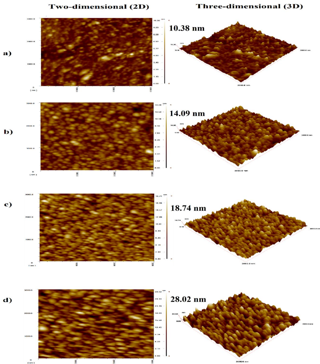
Figure 3. ZnS thin film AFM 2D and 3D images on Ge optical windows A) Ge without ZnS b) 3 mTorr Ge/ZnS c)20 mTorr Ge/ZnS d)30 mTorr Ge/ZnS
