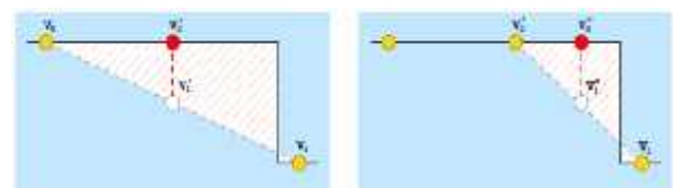
Figure 7. Over-refined triangle error on keen vertical faces
