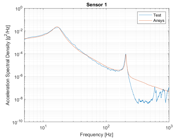
Figure 16. Sensor 1 Test vs ANSYS Comparison
