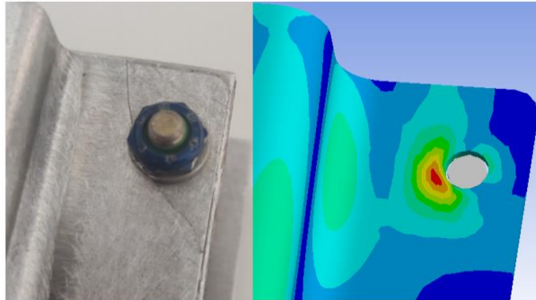
Figure 26. Fracture on the Mount and Finite Element Model
