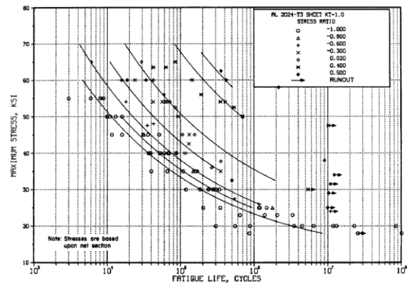
Figure 1. Unnotched 2024-T3 Aluminum Alloy S/N Curve [1]
