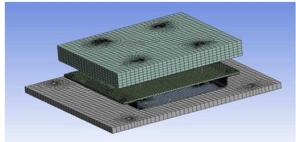
Figure 8. Meshed Model
