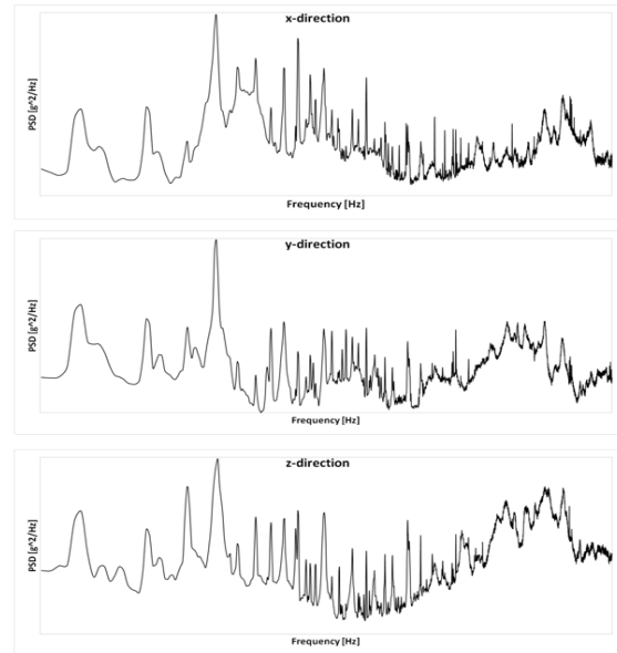
Figure 3. Acceleration PSD's
