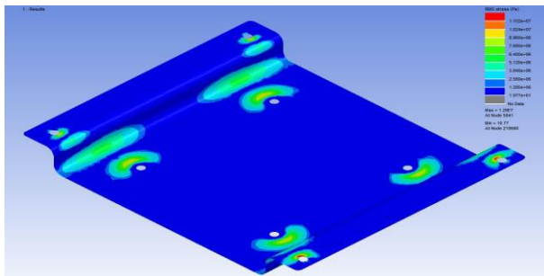
Figure 23. RMS Stesses for 2500 Hours Input PSD
