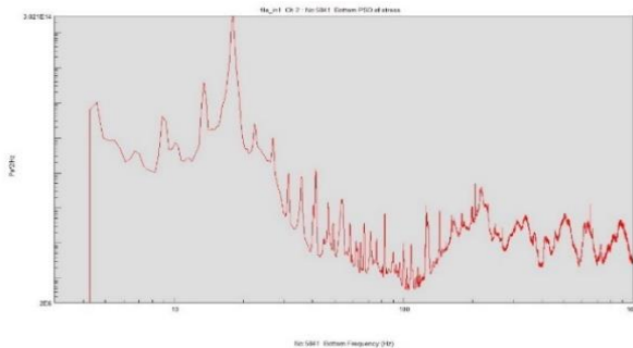
Figure 22. Stress PSD for 2500 Hours Input PSD
