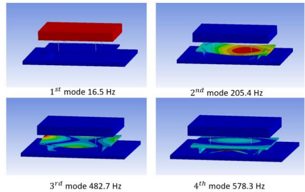
Figure 15. Mode Shapes of Structures
