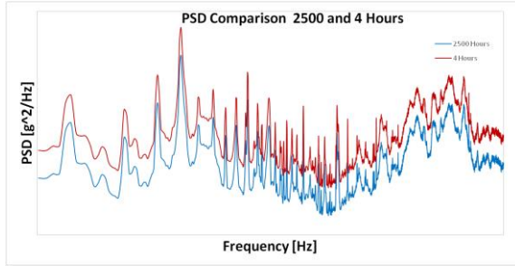
Figure 5. PSD Comparison for 2500 and 4 Hours
