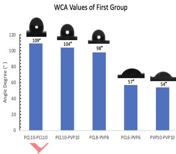
Figure 2. WCA values of PCL/PVP coaxial nanofibers with different core and shell polymer concentrations.
