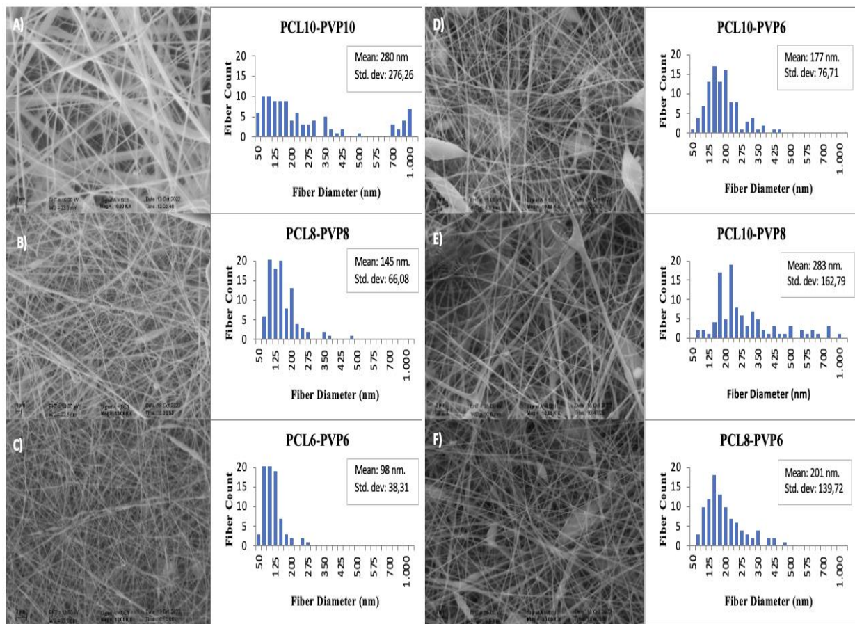
Figure 1. SEM images (at x10.000 magnifications) and fibre diameter distribution graphs of coaxial nanofibers A) PCL10–PVP10, B) PCL8–PVP8, C) PCL6–PVP6, D) PCL10–PVP6, E) PCL10–PVP8, F) PCL8–PVP6 samples, respectively.
