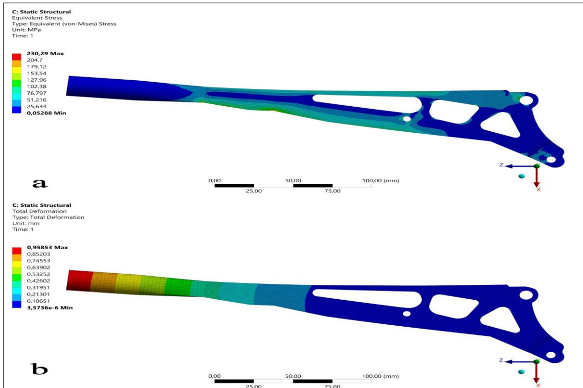
Figure 12. Result of static analyses of parking brake lever a) equivalent (von Mises) stress, b) total deformation
