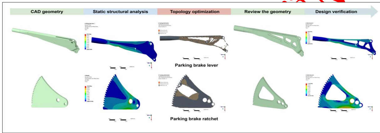
Figure. Topology optimization process flowchart
