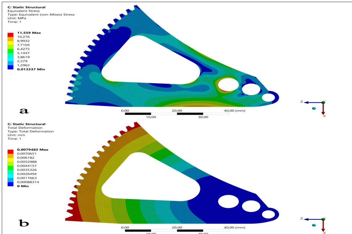
Figure 13. Result of static analyses of parking brake ratchet a) equivalent (von Mises) stress, b) total deformation
