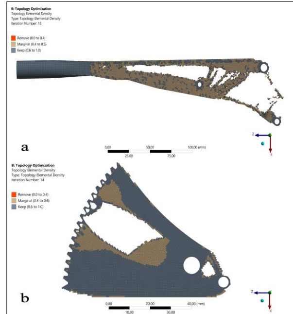
Figure 10. Occurred geometries after topology optimization a) parking brake lever, b) parking brake ratchet
