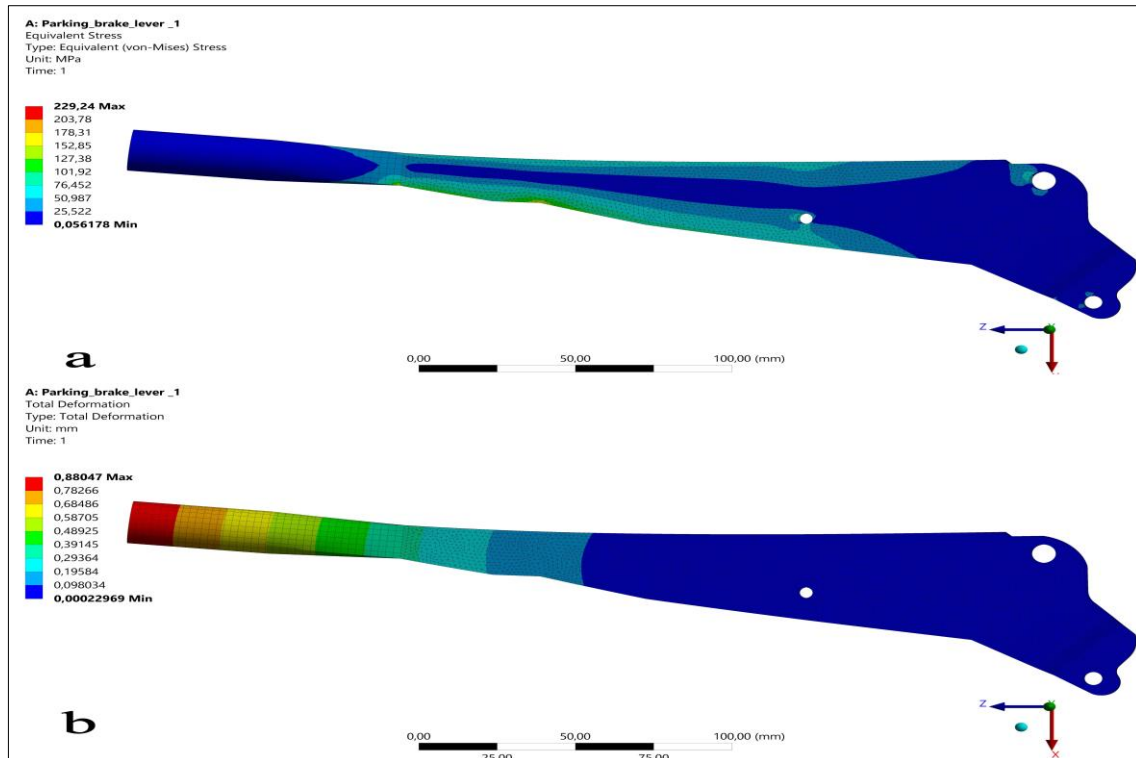
Figure 8. Result of static analyses of parking brake lever a) equivalent (von Mises) stress, b) total deformation
