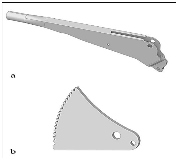
Figure 4. CAD models a) parking brake lever, b) parking brake ratchet
