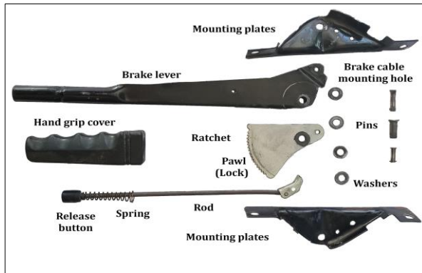
Figure 3. Parking brake lever mechanism parts
