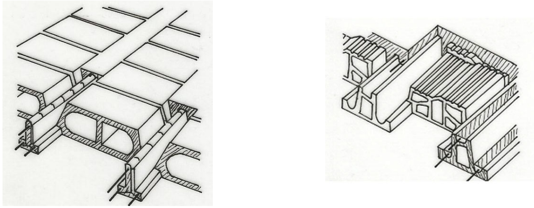
b. Slab assembly consisting of prefabricated reinforced concrete voided beam and hollow brick components.
