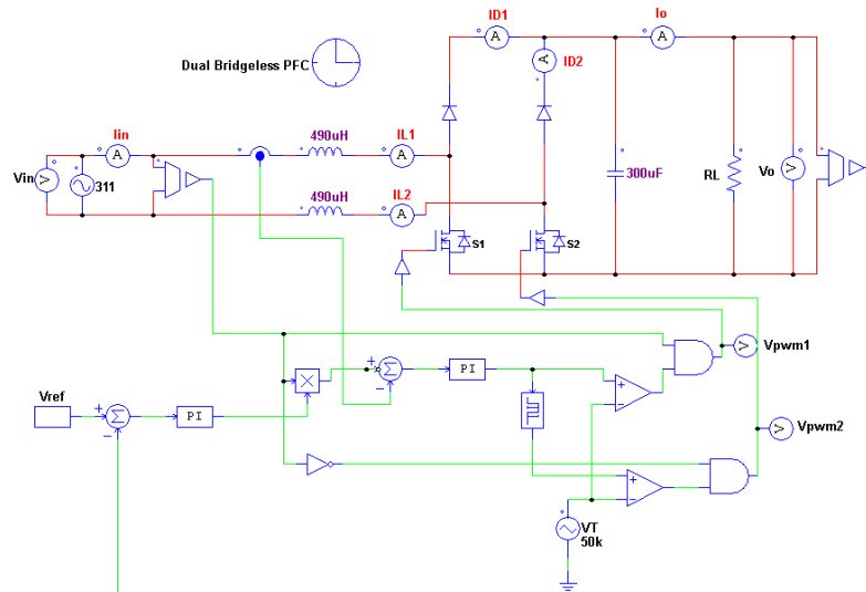
Figure 7. Simulation model of D-BBPFC Converter
