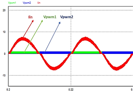
Figure 8. I_{in} and control signals of S_1 - S_2
