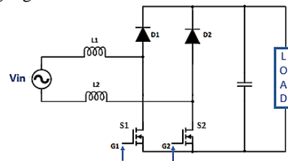
Figure 5. Circuit of the D-BBPFC Converter
