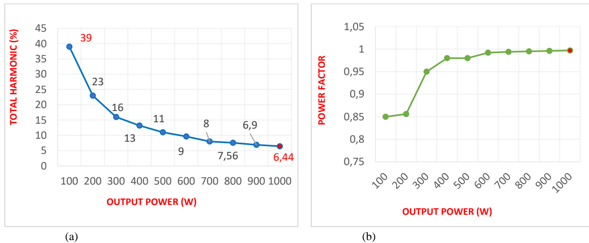
Figure 10. a) THD b) power factor of Dual-Boost Bridgeless PFC at 10%-100% output power
