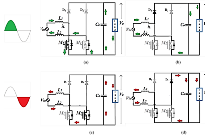
Figure 6. a) M_1 is ON b) M_1 is OFF in positive half-period c) M_2 is ON d) M_2 is OFF in negative half-period
