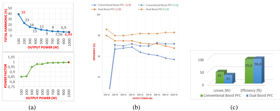
Figure. a) The change of power factor and harmonic distortion b) detailed efficiency analysis c) comparison of losses and efficiency of converters
