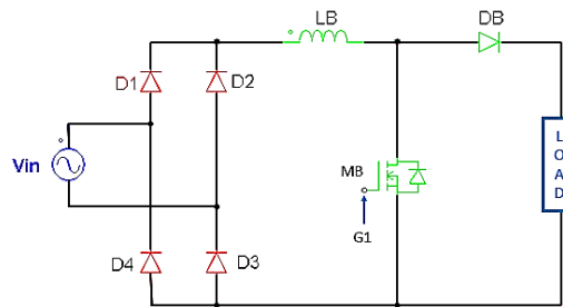
Figure 1. Circuit of the CBPFC Converter
