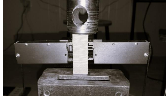
Figure 2. Compression test using bi-axial extensometer.
