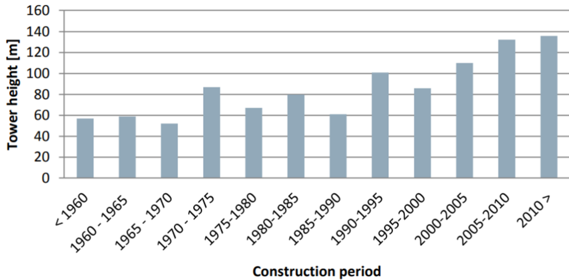
Figure 3. Maximum tower height development (Hartmann, 2014)
