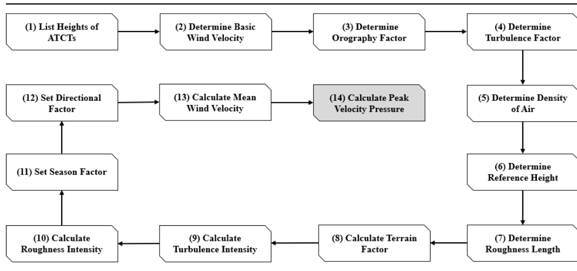
Figure 6. Calculating peak velocity pressure flow chart
