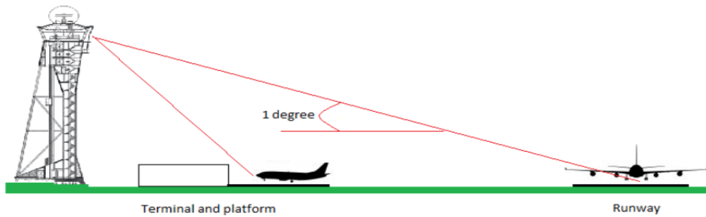
Figure 1. Minimum line of sight and direct visibility on active pavement (Hartmann, 2014)
