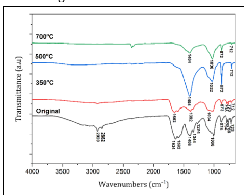
Figure 3. FT-IR results of PM.
