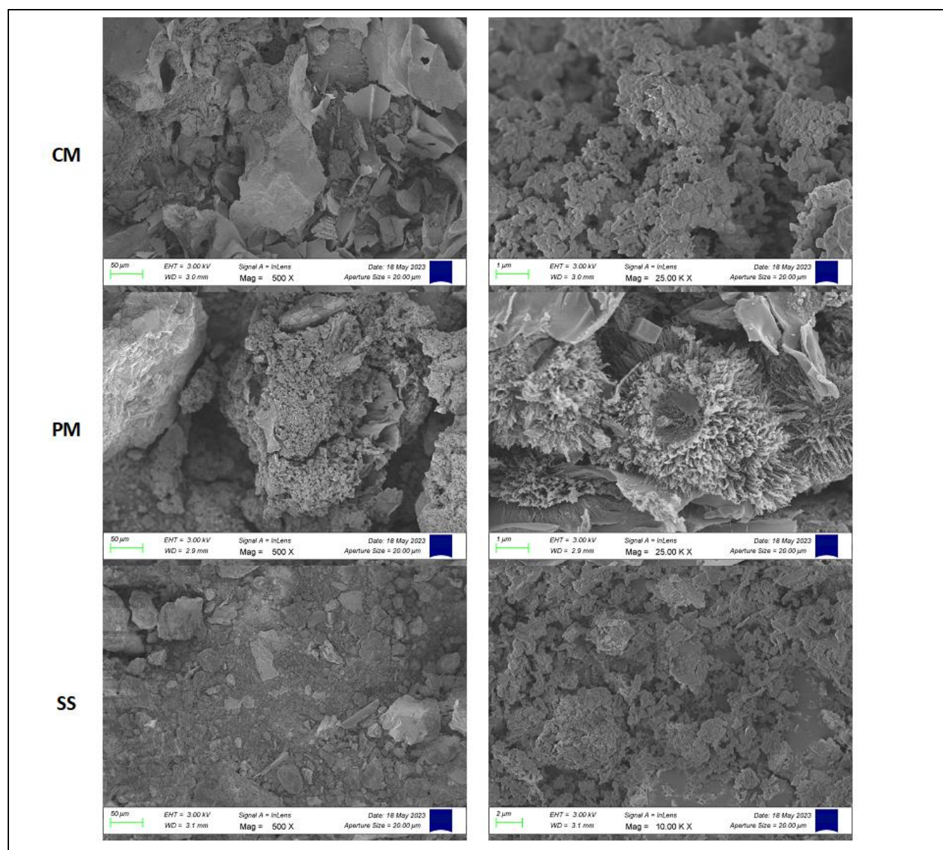
Figure 5. SEM images of CM, PM and SS at 700 °C.
