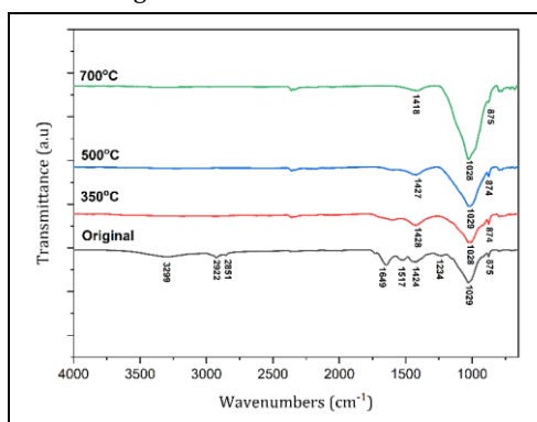
Figure 4. FT-IR results of SS.
