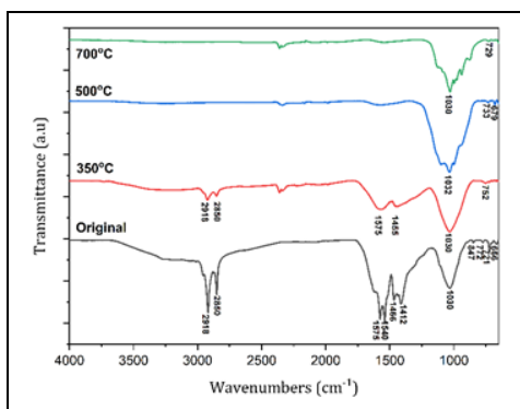
Figure 2. FT-IR results of CM.
