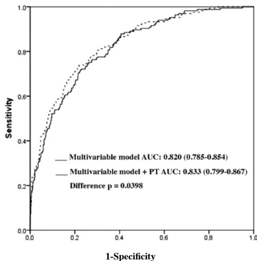
Figure 2. Receiver operating characteristic (ROC) curves for the multivariable model and multivariable model plus prothrombin time (PT) for predicting all-cause total mortality.
