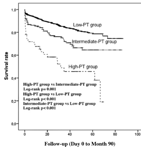
Figure 3. Kaplan-Meier survival curves for all-cause mortality.
