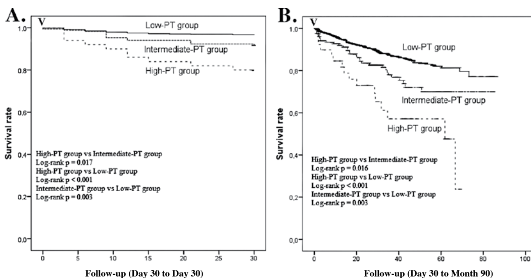
Figure 4. Landmark analysis: cumulative survival rate during the first 30 days after diagnosis of acute coronary syndrome (A) and after 30 days (B).
