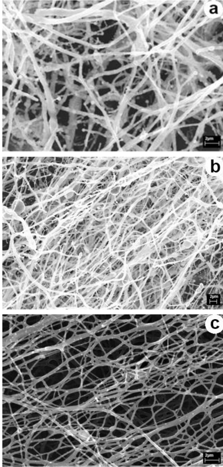
Figure 6: SEM images of Strontium aluminate nanofibers (10 kX) (a) SrO.Al 2 O 3 .xB 2 O 3 (Eu, Dy) x=0 (b) SrO.Al 2 O 3 .xB 2 O 3 (Eu, Dy) x=0.2 (c) SrO.Al 2 O 3 .xB 2 O 3 (Eu, Dy) x=0.4.
